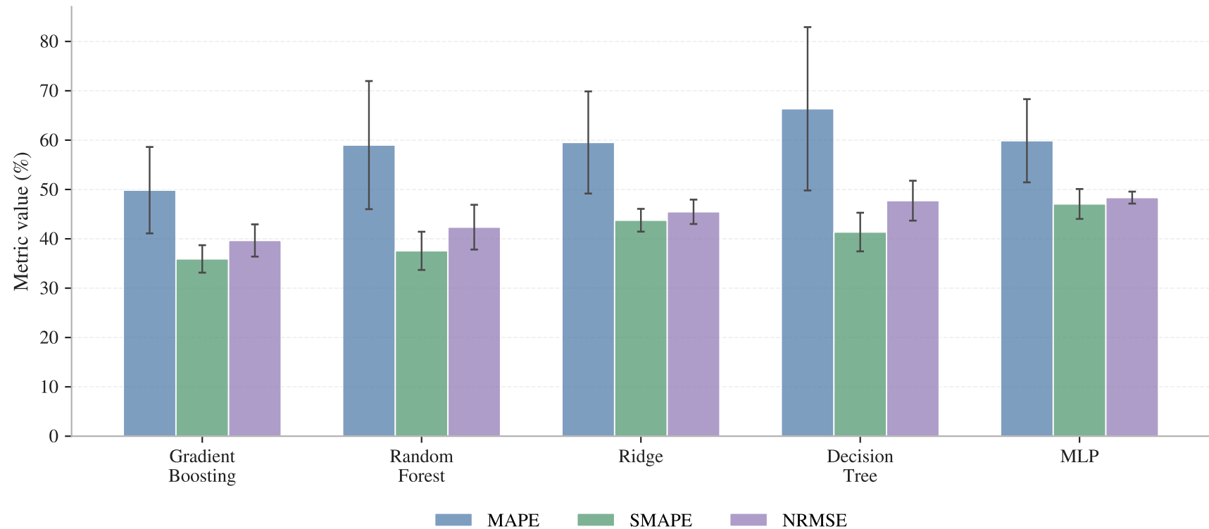
Supplementary dimensionless error metrics
