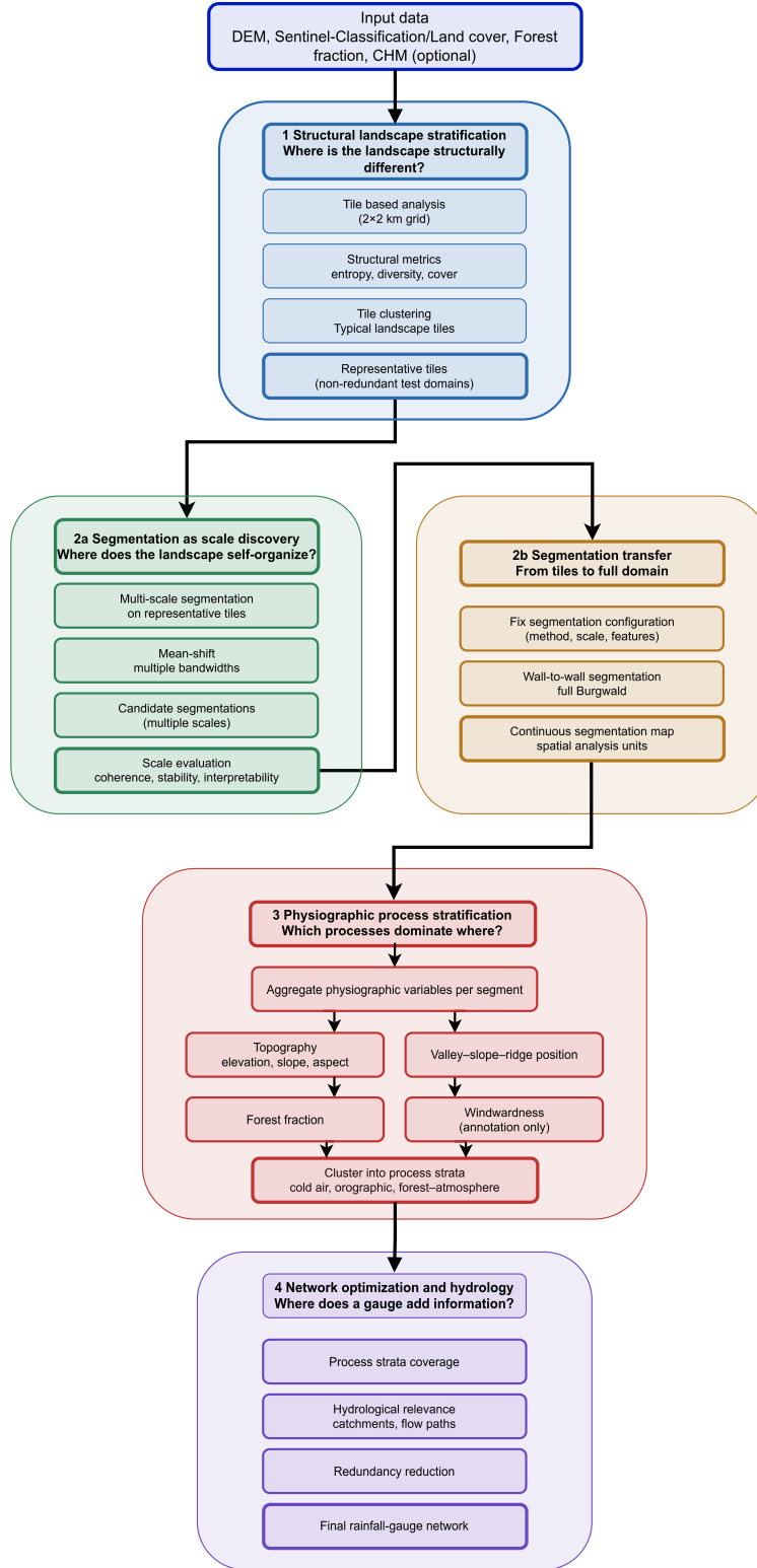
Figure 1: Design framework for the Burgwald rainfall gauge network
