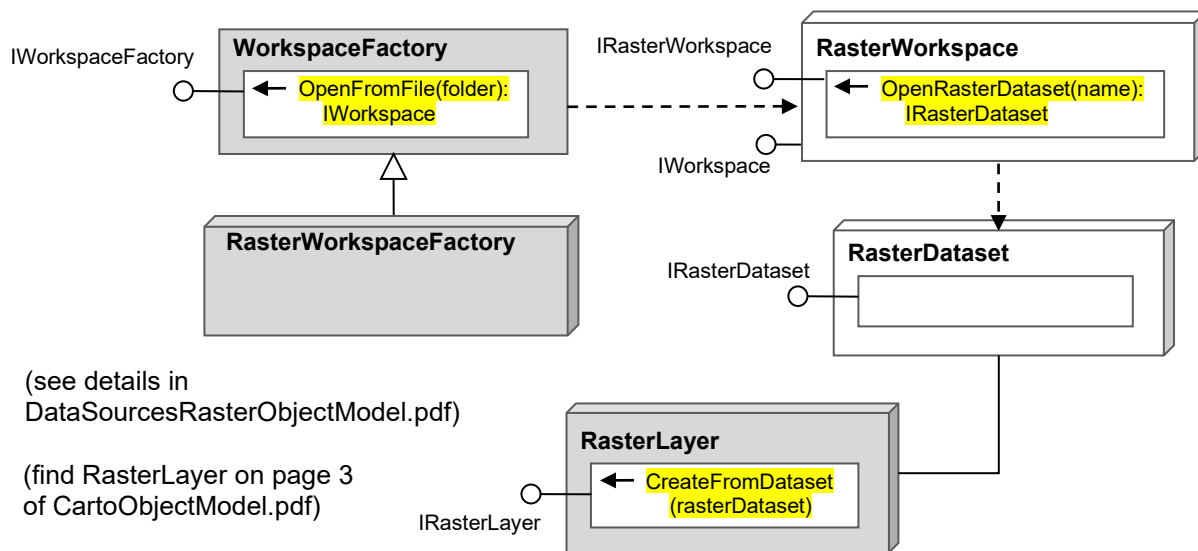
Figure 5 Object model diagram for creating raster datasets and raster layers
