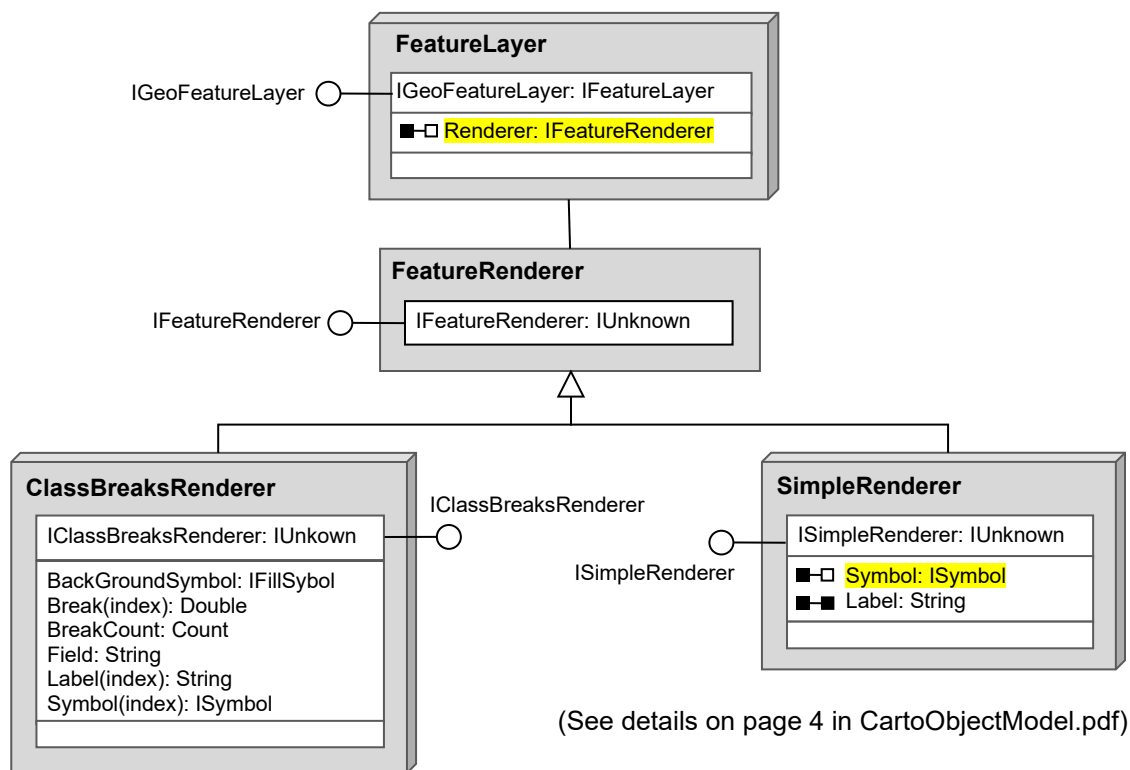
Figure 6 Object model diagram for rendering feature layers
