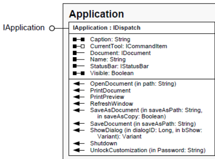
Figure 3 Part of the Application component
