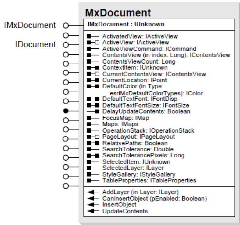
Figure 4 Part of the MxDocument component
