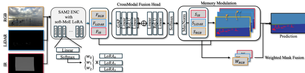
Figure 1. Overview of GatedMemorySAM. Each modality is encoded by SAM2 with Soft-MoE LoRA, scored by the CrossModalFusionHead, and fused via memory modulation and weighted mask fusion.
