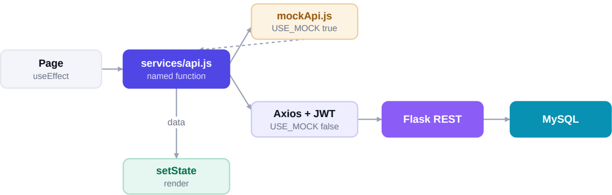
Figure 3 - One gateway, two possible backends, identical response shape.
