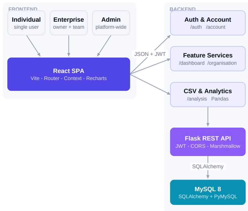
Figure 1 - System architecture. The frontend never reaches the database directly.
