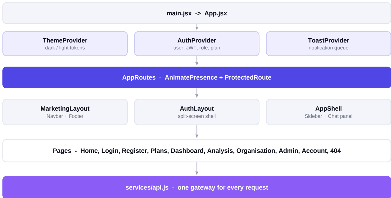
Figure 2 - Frontend composition, outermost layer at the top.
