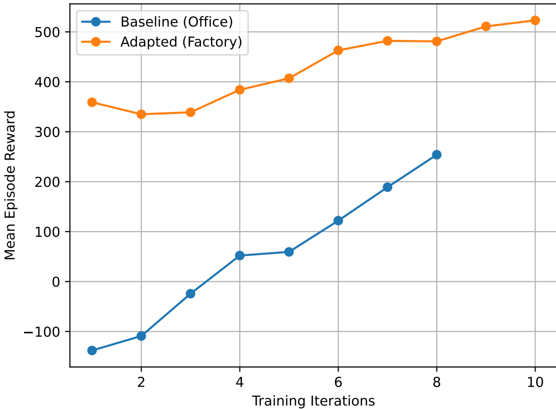
Figure 4.1: PPO Training Curve
