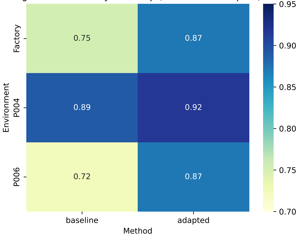
Figure 4.7: Accuracy Heatmap (Baseline vs Adapted)
