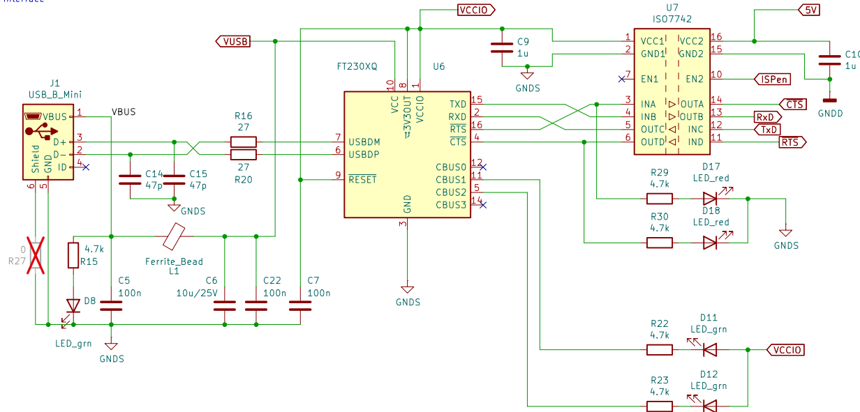
USB interface
