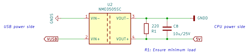
Isolated DC/DC conversion
