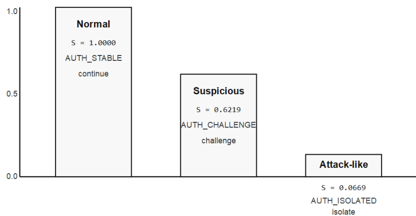
Figure 3: PoC stability results for normal, suspicious, and attack-like sessions.
