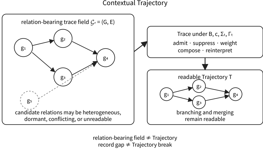
Figure 3: Contextual tracing from a relation-bearing field to a readable Trajectory.
