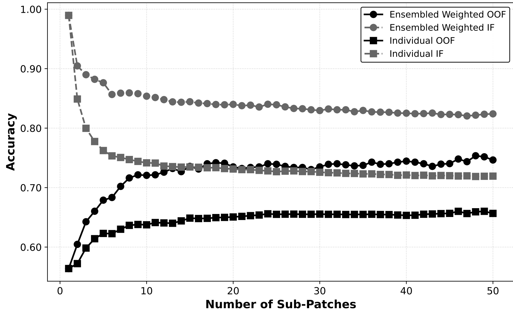
Performance Comparison: OOF vs IF
