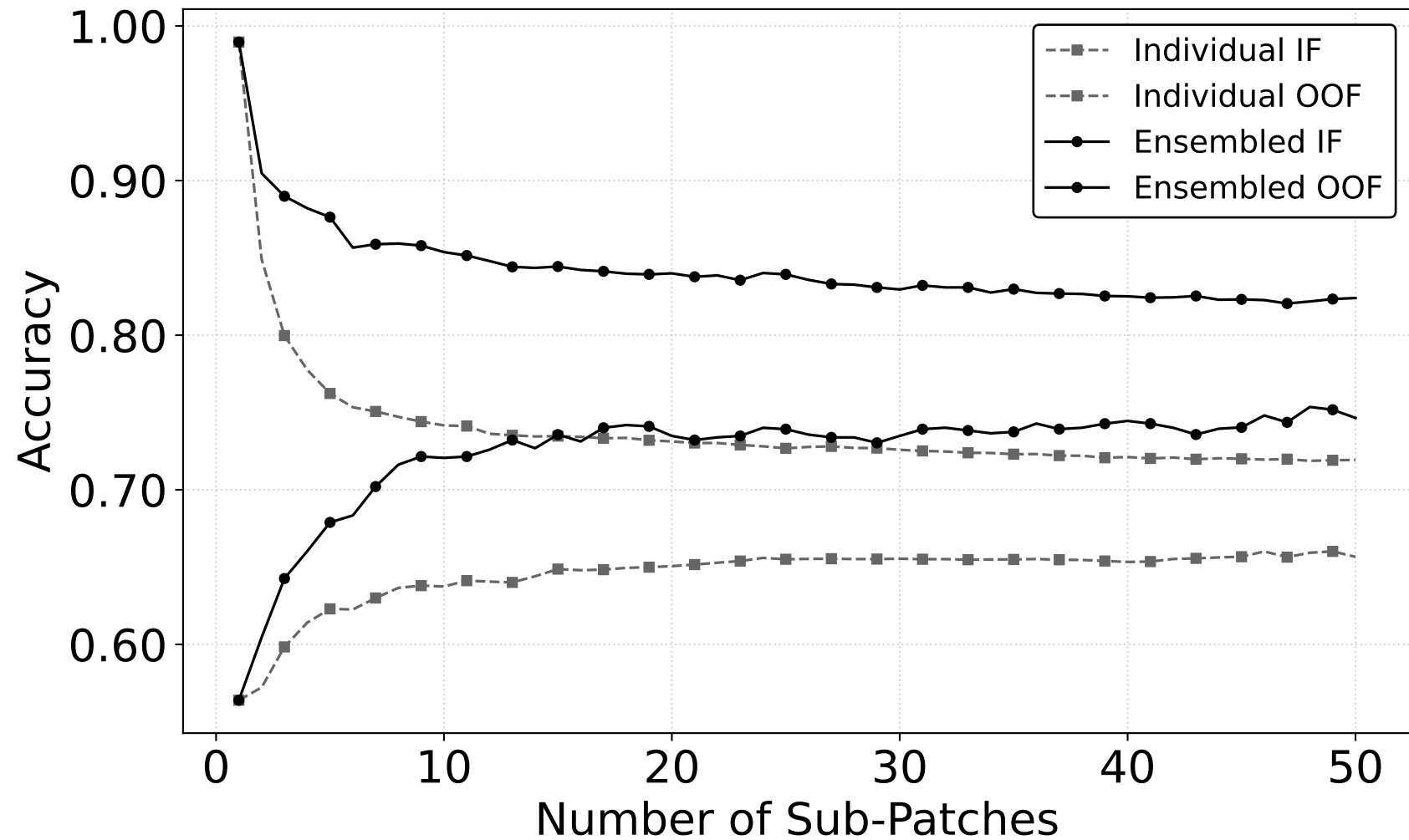
Accuracy vs Patch Number
