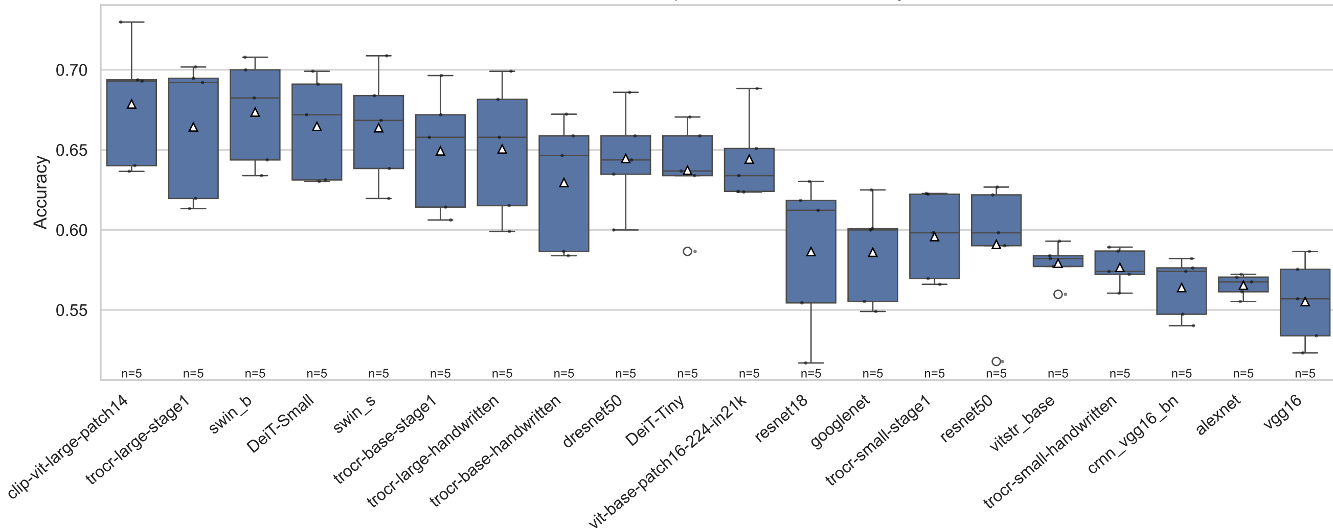
Distribution of Accuracies per FE Model, standard body dataset
