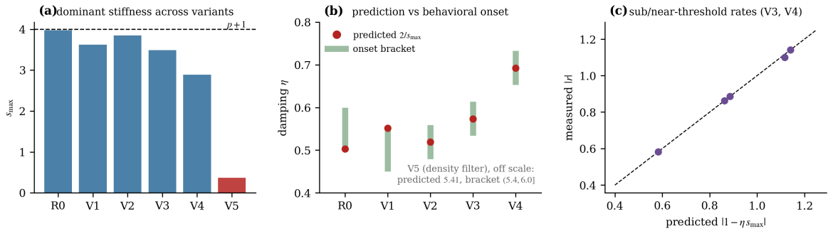
Figure 6: Robustness of the threshold law (Section 5.1, Table 1). (a) s_{\max} across variants; the density filter (V5) collapses it to 0.37. (b) predicted 2/s_{\max} versus behavioral onset brackets for R0–V4 (V5 off scale: predicted 5.41, bracket (5.4, 6.0]). (c) flip-active probe rates versus |1 - \eta s_{\max}| on V3/V4—three-decimal agreement below threshold.
