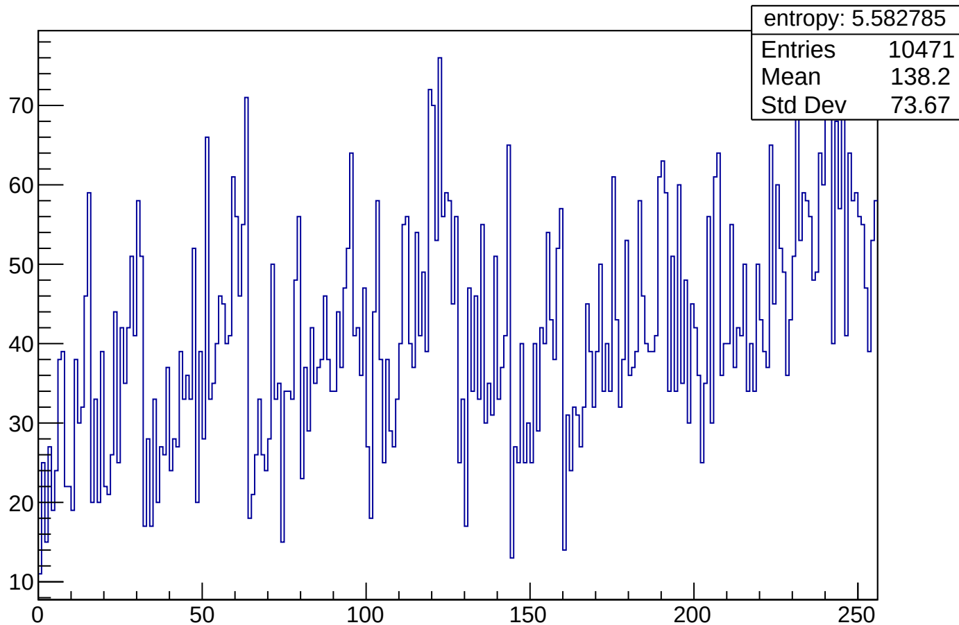
exponential_Z_BEST_COMPRESSION_round_1000_bytes
