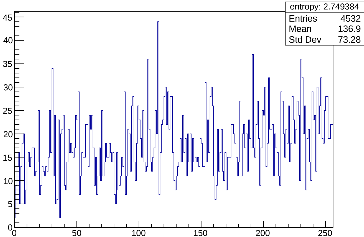
exponential_Z_BEST_COMPRESSION_round_16_bytes
