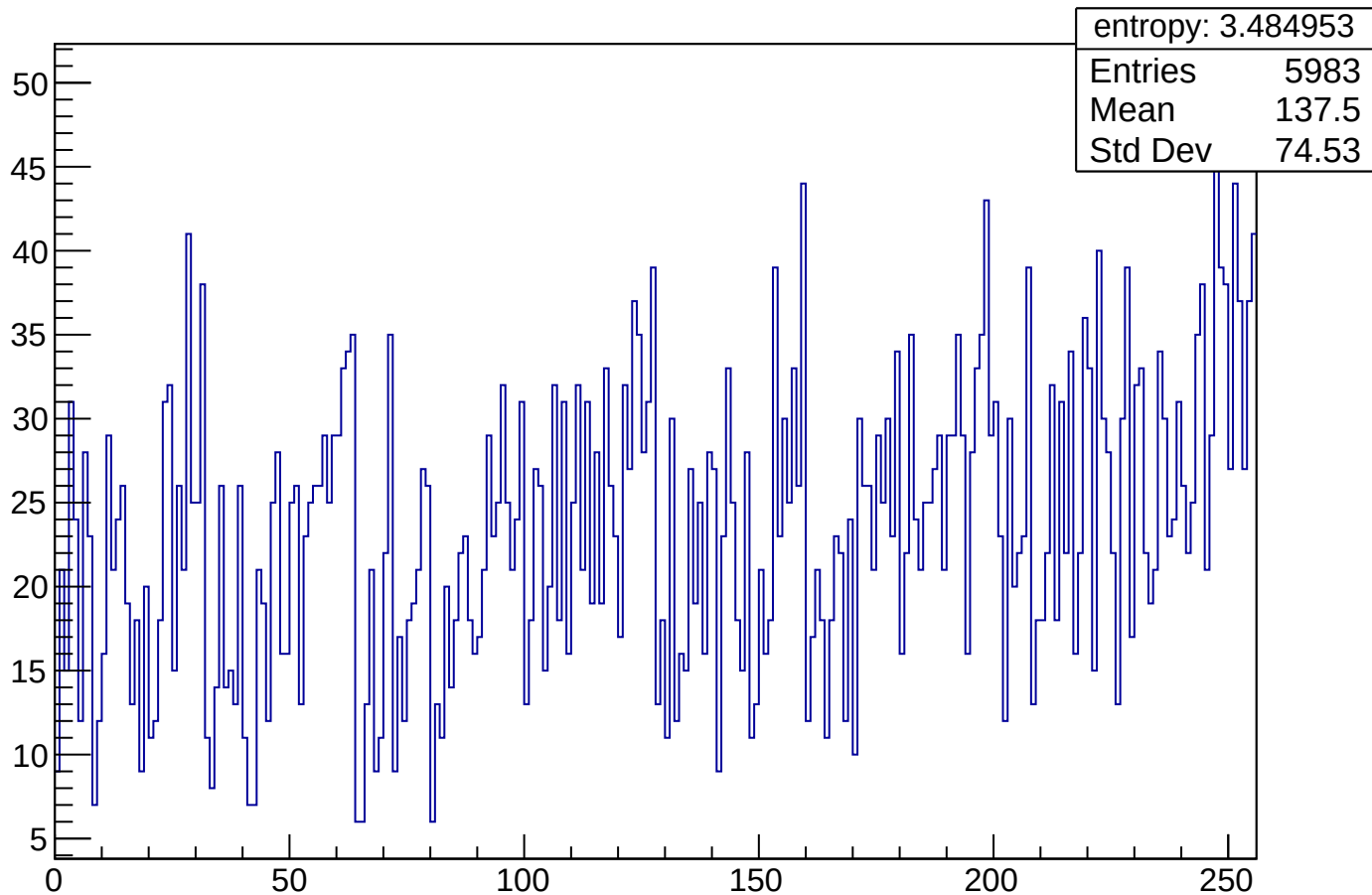
exponential_Z_BEST_COMPRESSION_round_64_bytes
