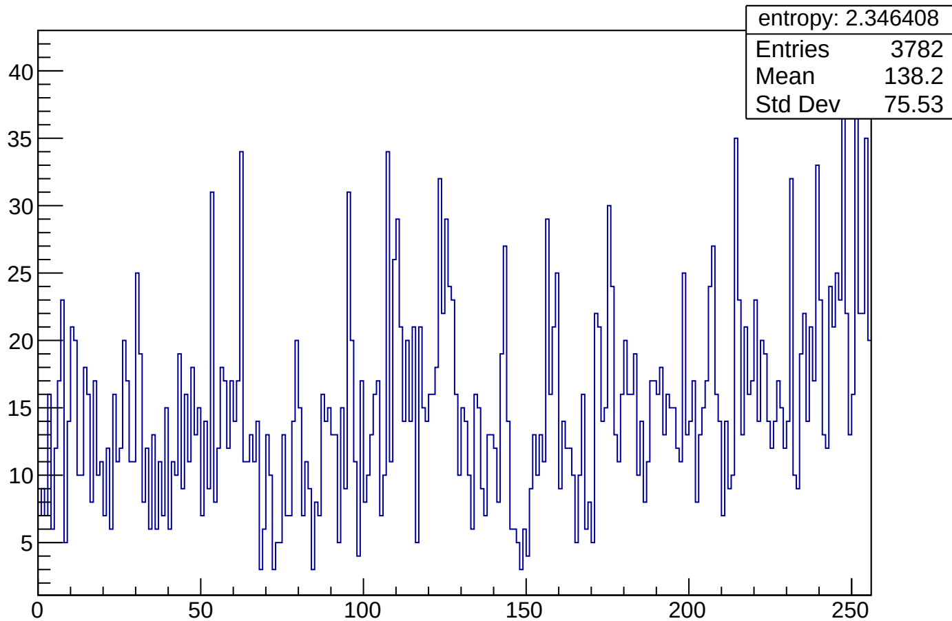
exponential_Z_BEST_COMPRESSION_round_8_bytes
