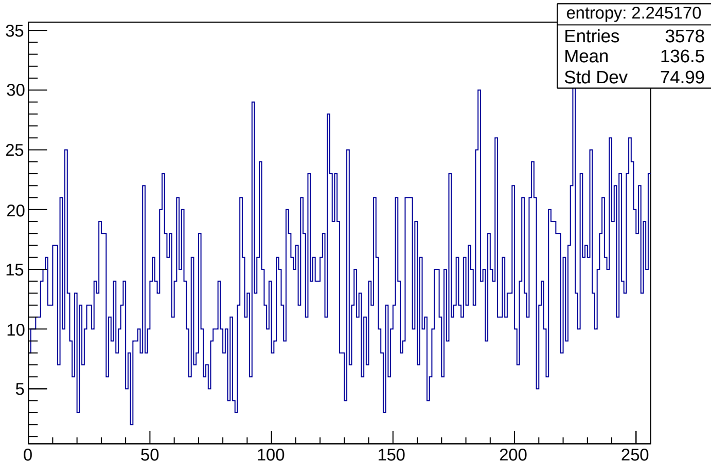
uniform_Z_BEST_COMPRESSION_round_2_bytes
