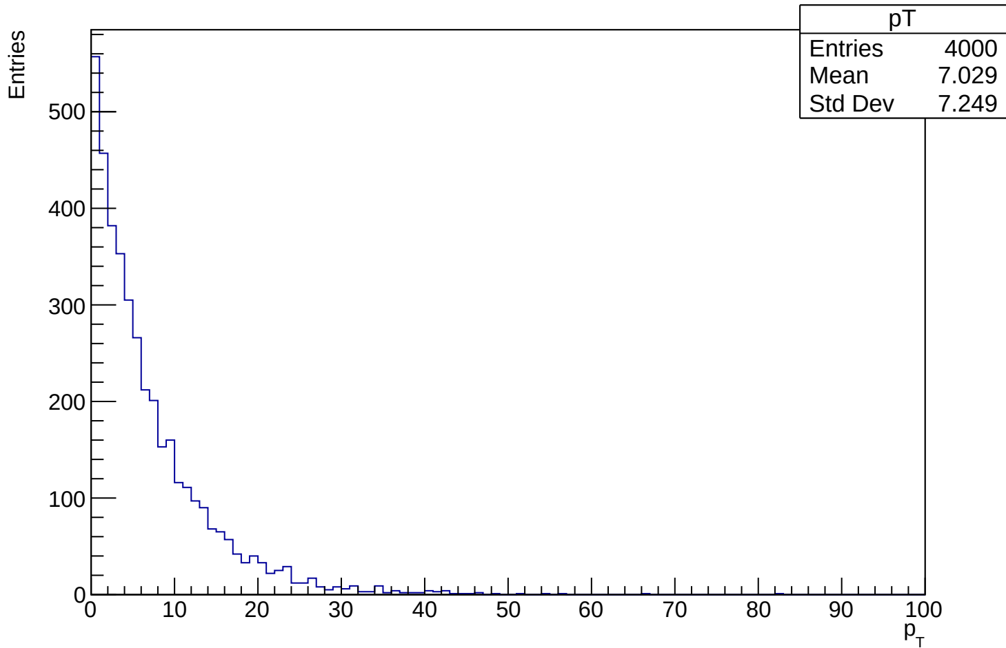
Distribution of pT values rounded
