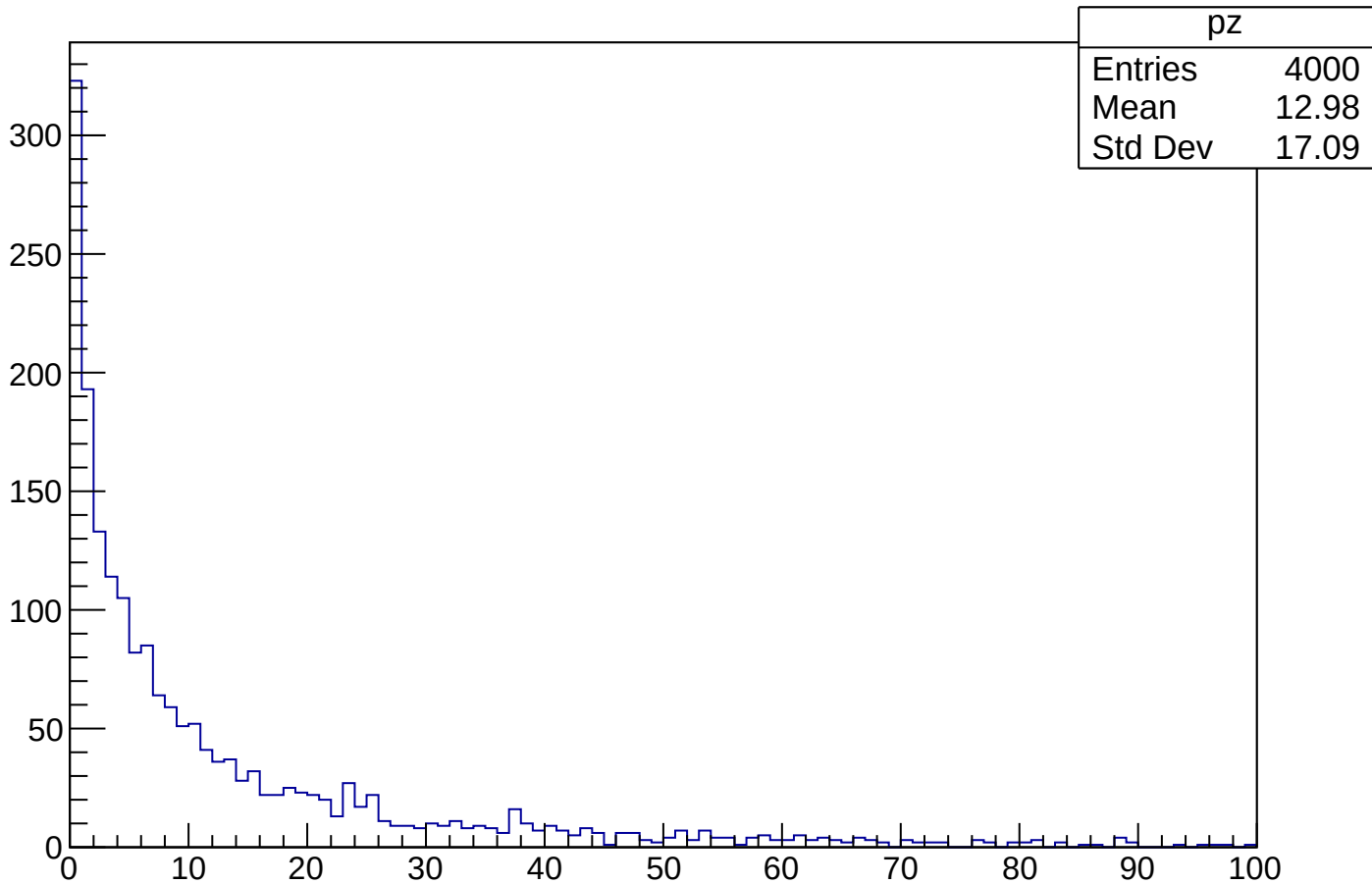
Distribution of pz values default
