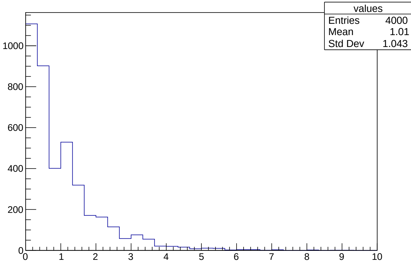
exponential_Z_BEST_COMPRESSION_round_8_values
