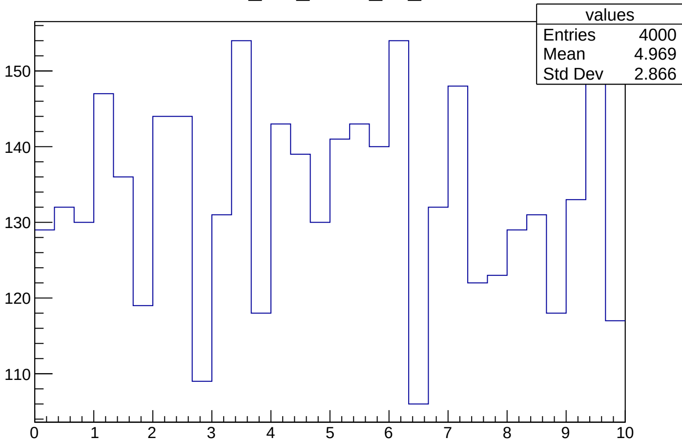
uniform_NO_round_32_values
