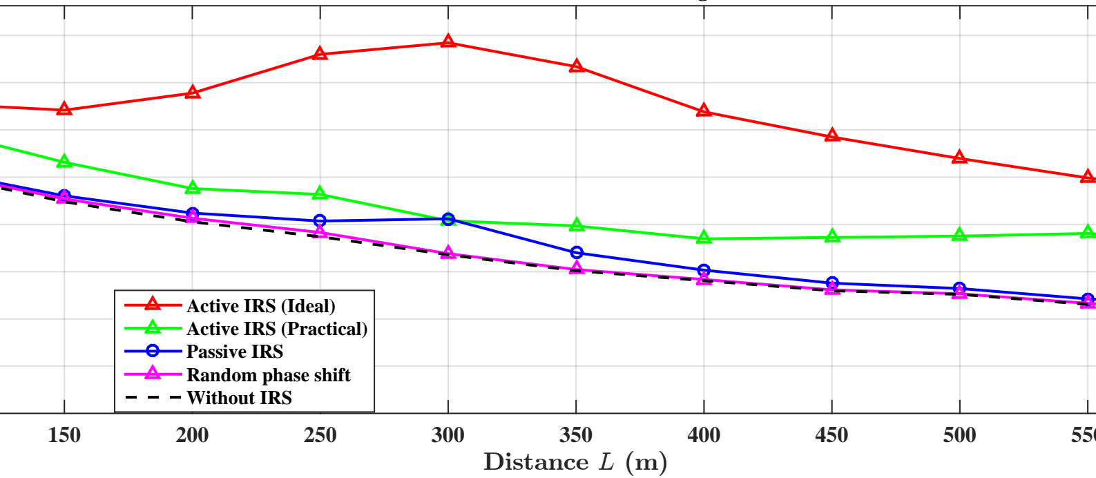
Sum-Rate Vs Distance (Strong LoS)
