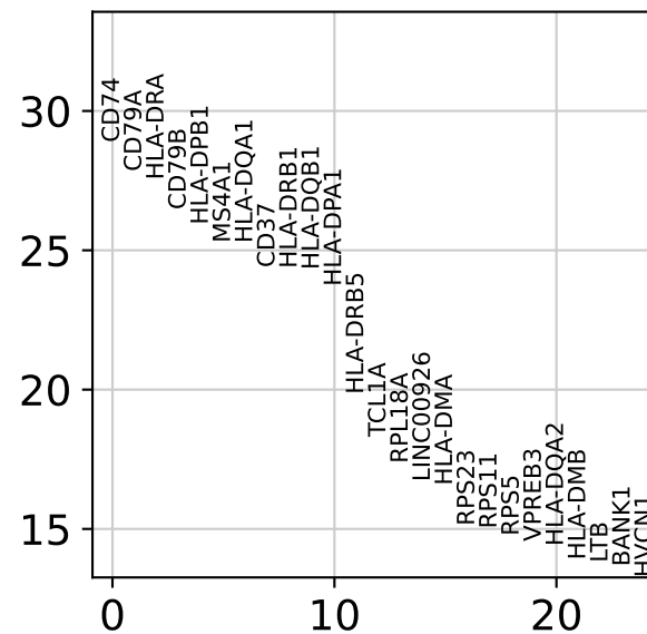
2 vs. rest
