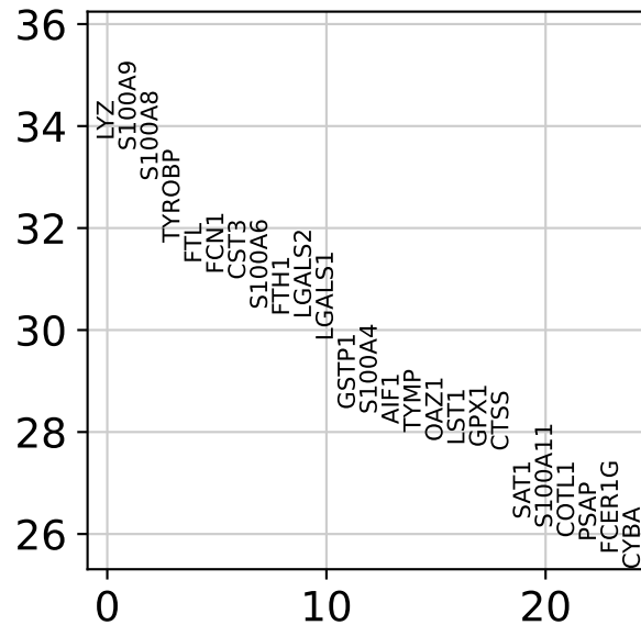
1 vs. rest
