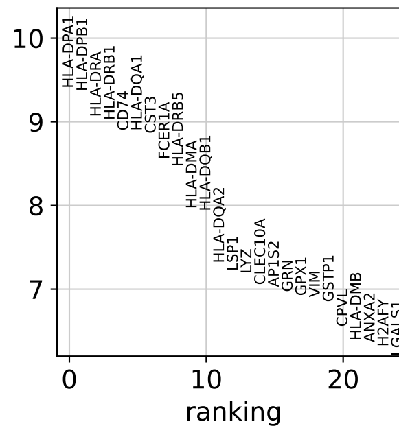
6 vs. rest
