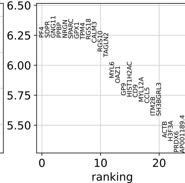
7 vs. rest
