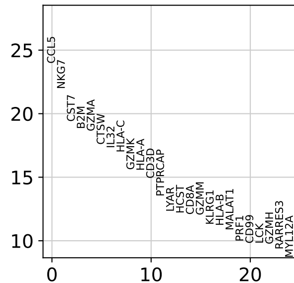
3 vs. rest
