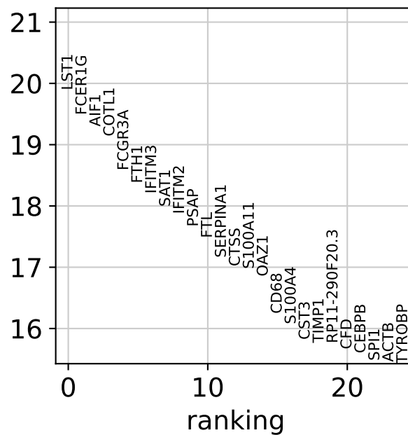
5 vs. rest
