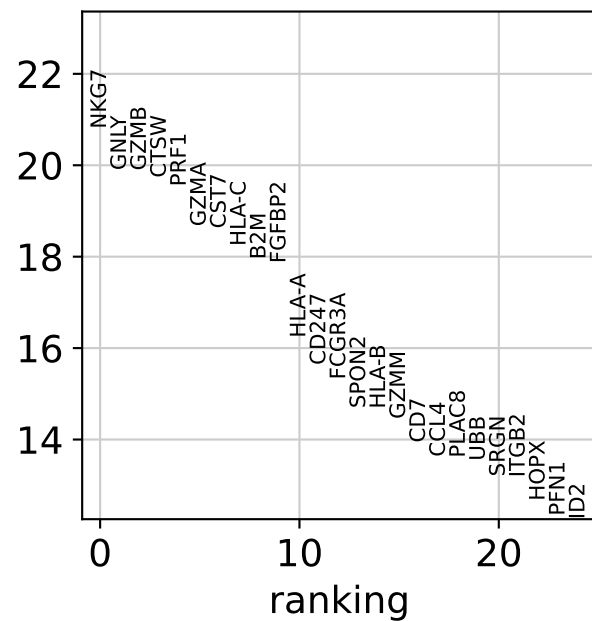
4 vs. rest
