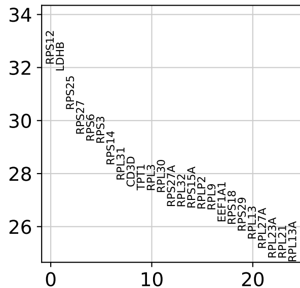
0 vs. rest
