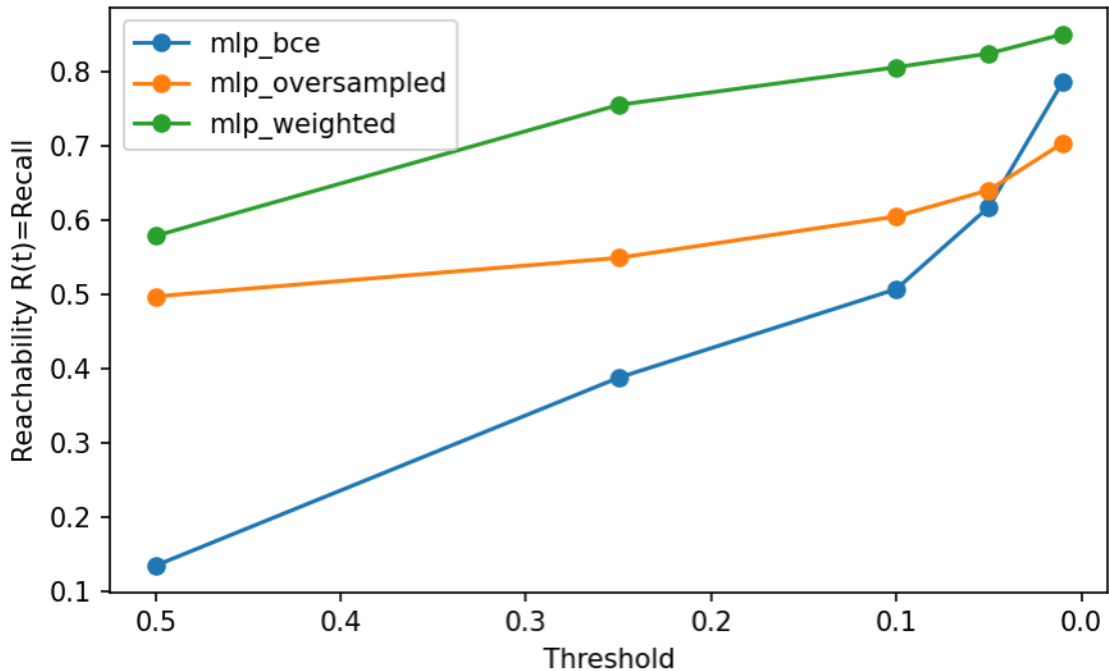
MLP Reachability Transition
