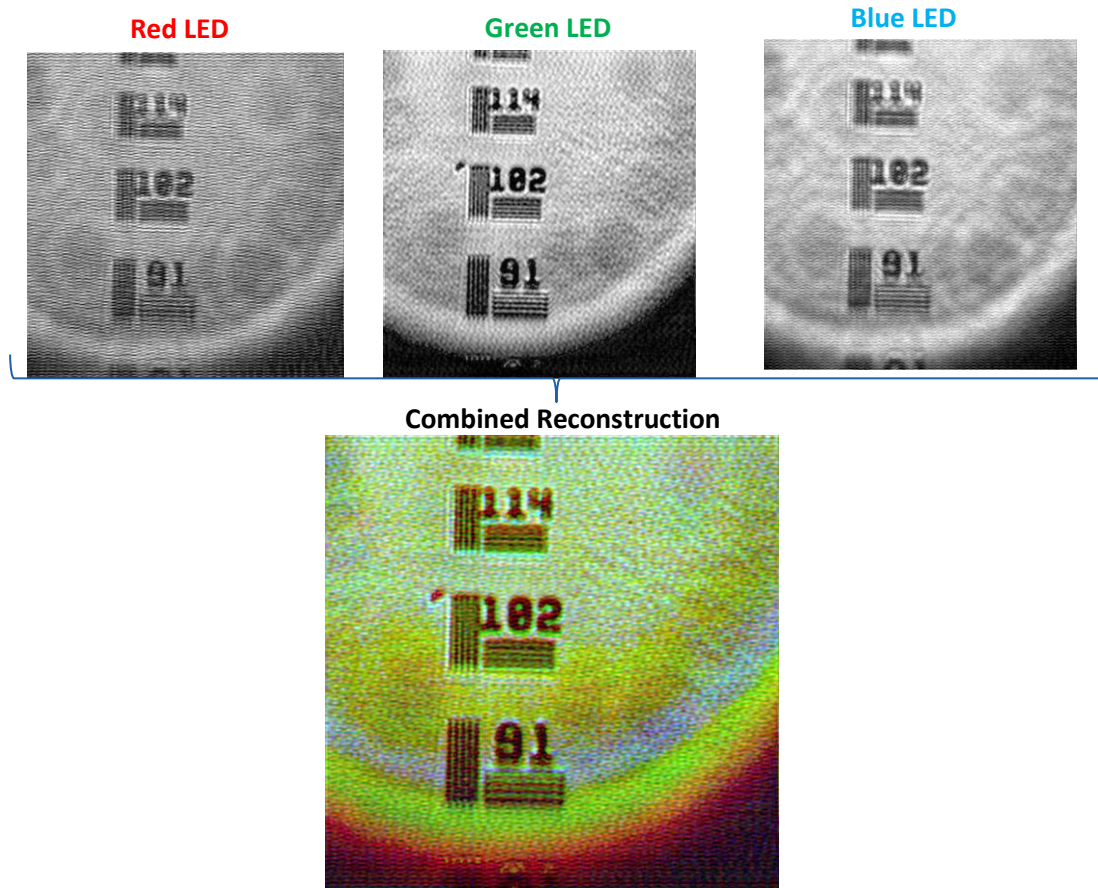
Figure 6.Second Reconstruction(USAF Chasrt)
