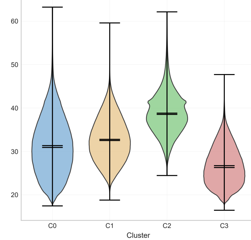
(h) Maximum log10(Nw)
