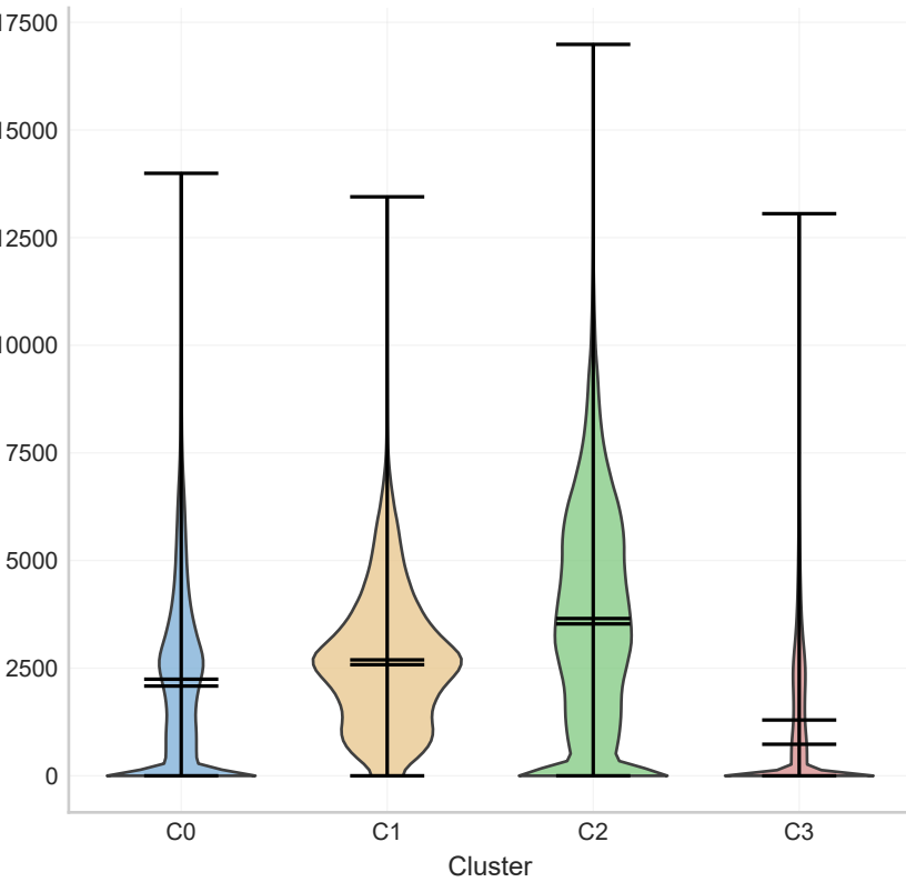
(e) Ice-phase layer depth
