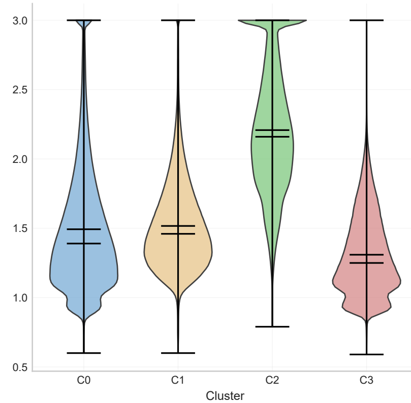
(g) Maximum Dm
