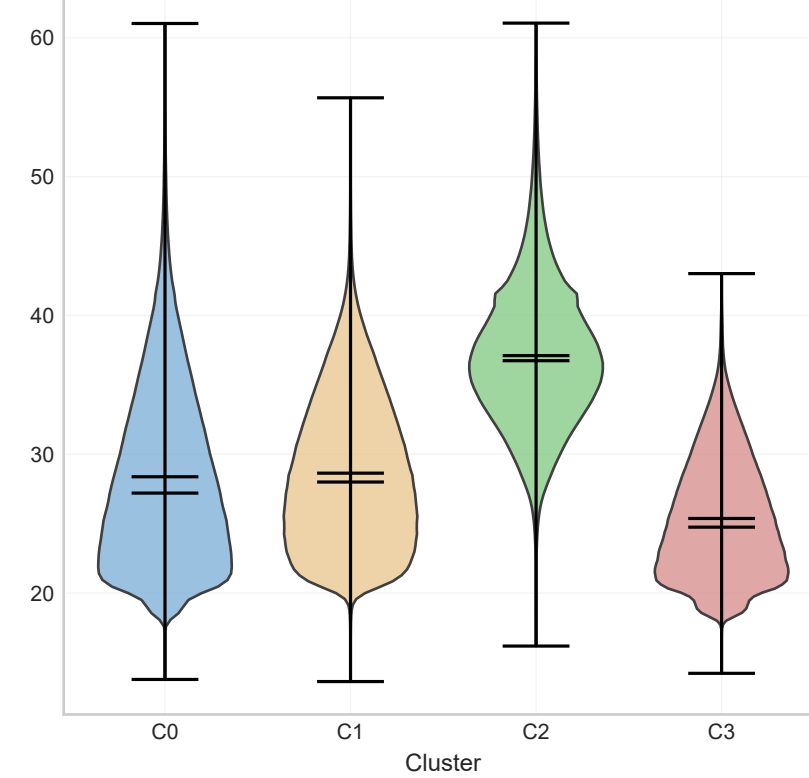
(g) Maximum Dm
