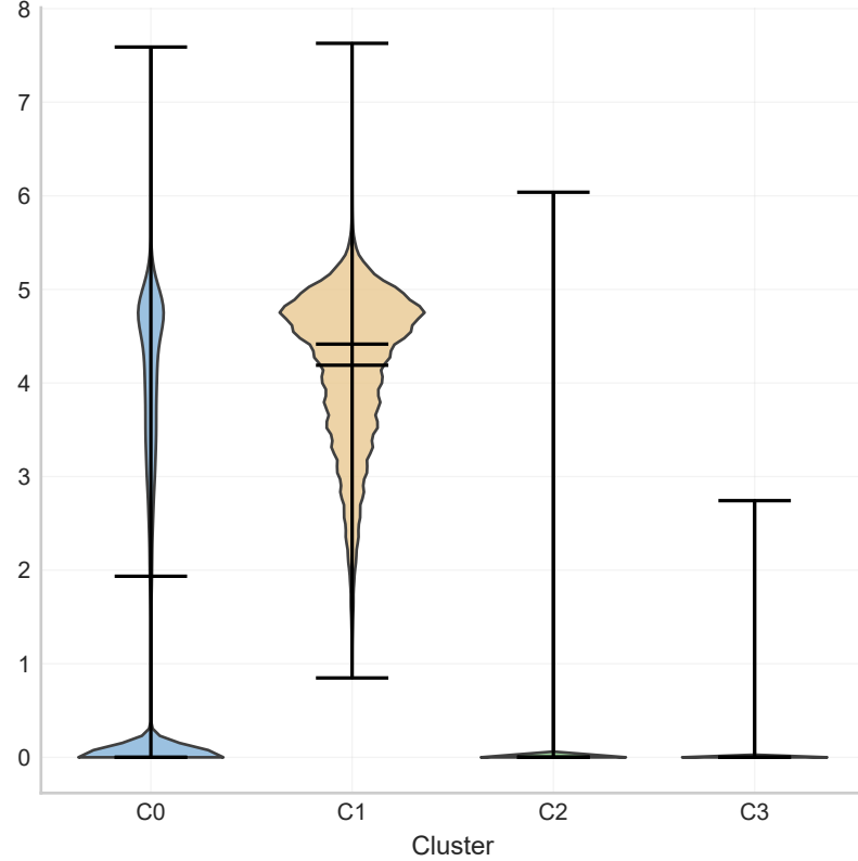
(f) Bright-band height
