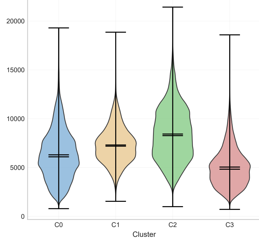
(f) Bright-band height
