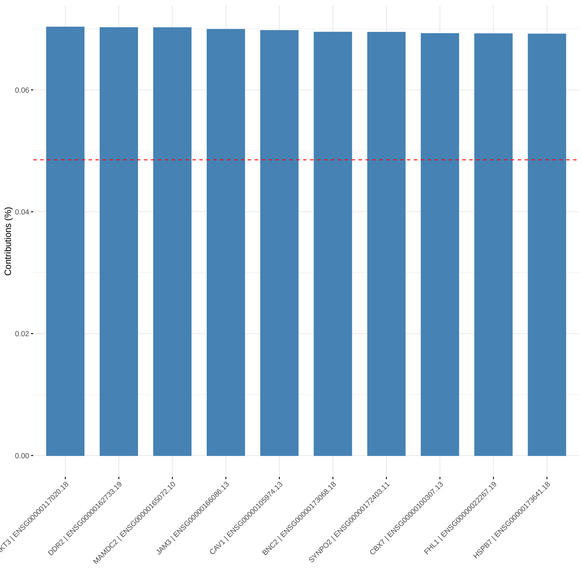
Contribution of variables to Dim-1-2
