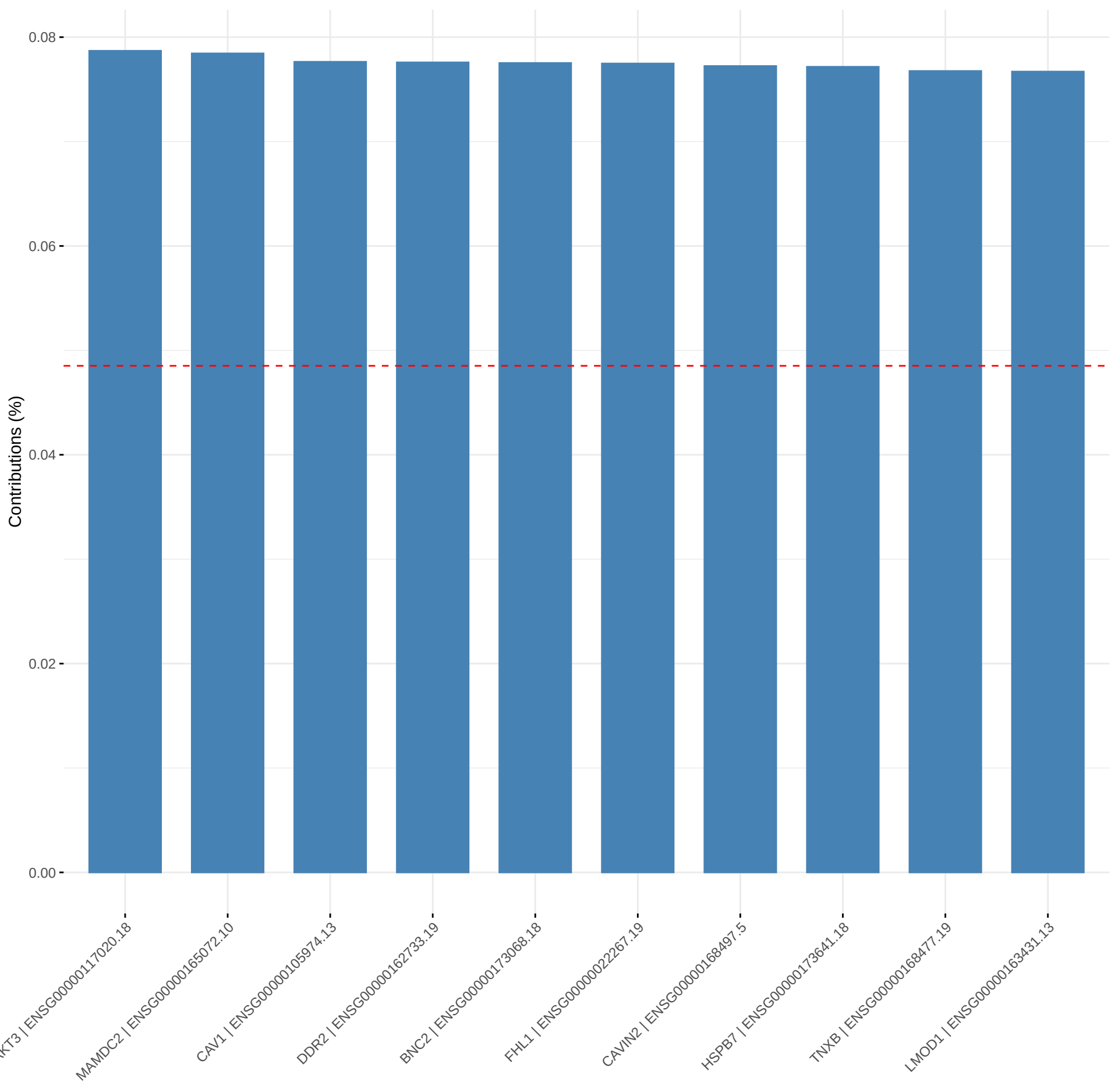
Contribution of variables to Dim-1
