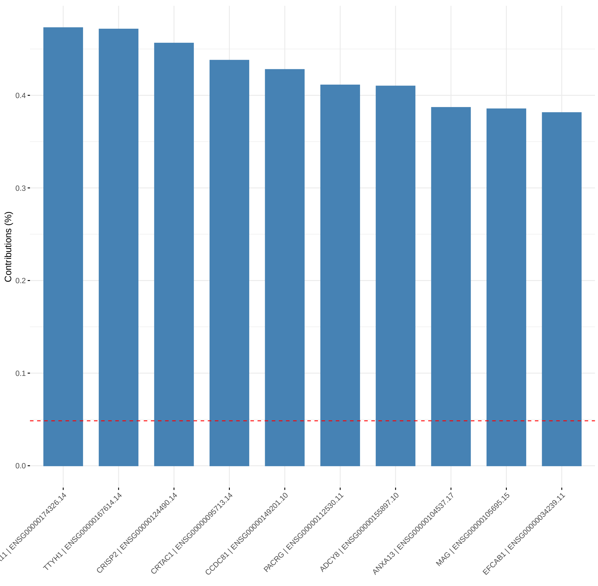
Contribution of variables to Dim-2
