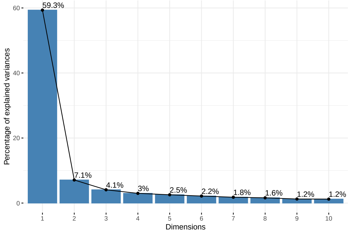
Scree plot
