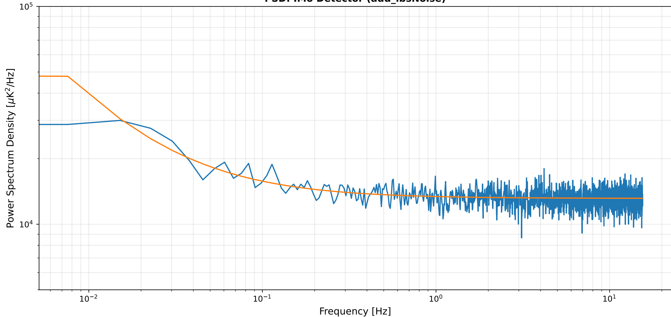
PSD: IMo Detector (add_lbsNoise)
