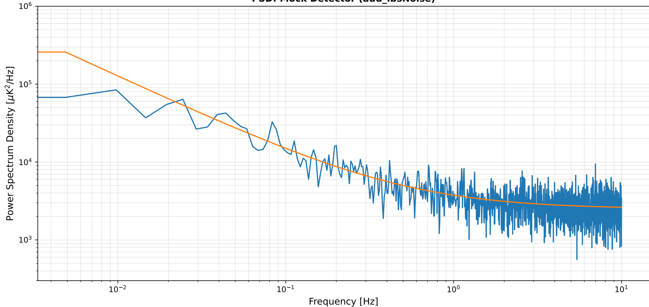
PSD: Mock Detector (add_lbsNoise)
