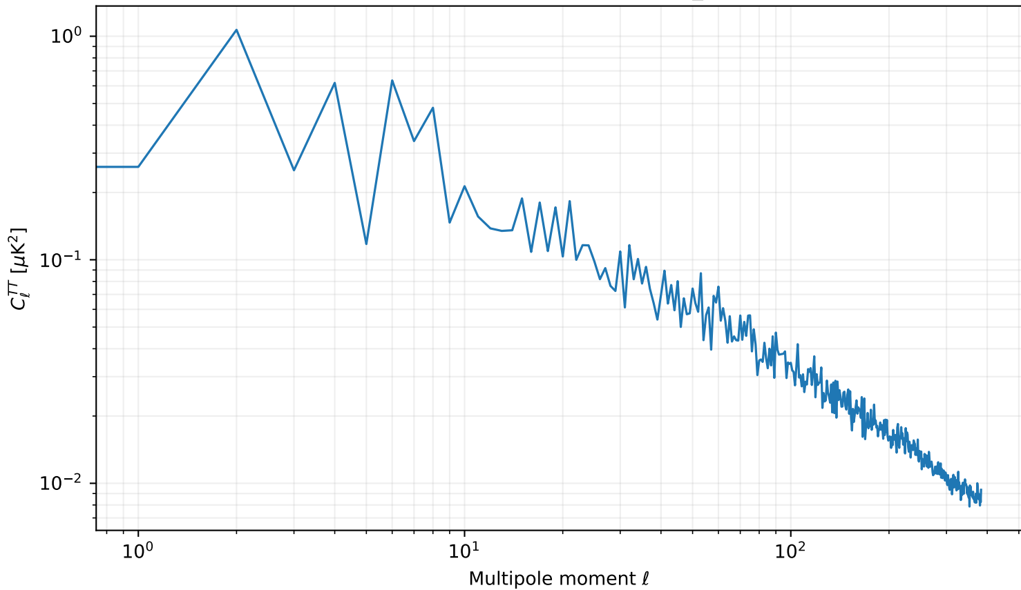
Angular Power Spectrum - add_lbsNoise
