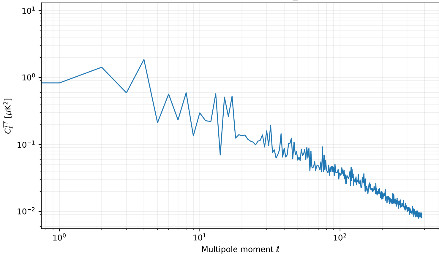
Angular Power Spectrum - add_OofaNoise
