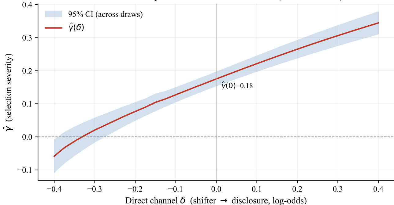
Selection severity under a direct shifter channel (100 MC draws)
