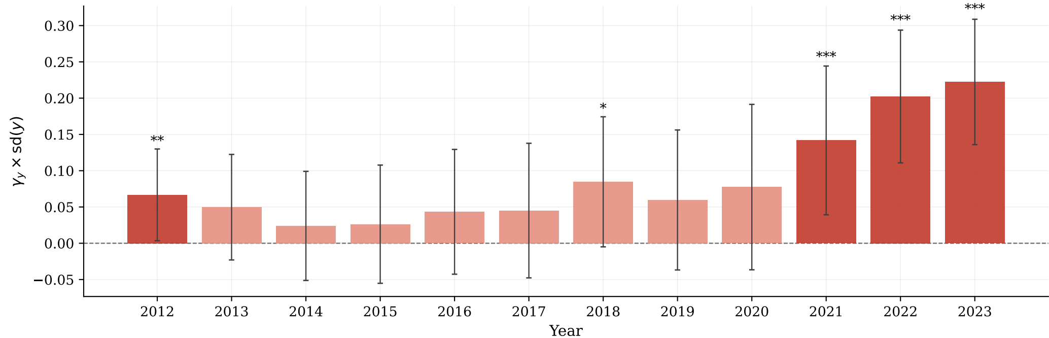
Selection Severity by Year: Propensity model with emissions \times year interactions
