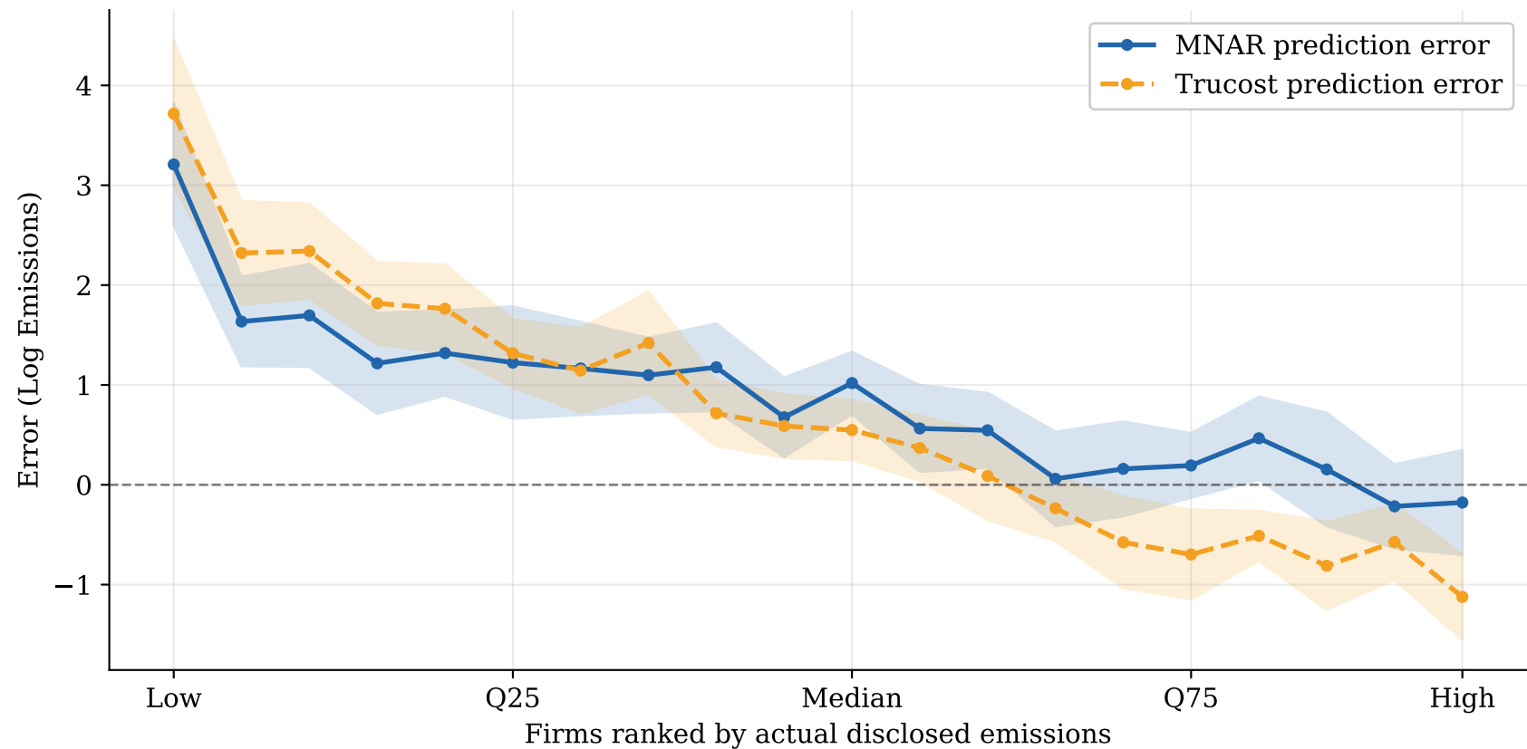
Prediction Error by Emission Quantile (prediction at t - 1 vs actual at t = 0 , 95% CI)
