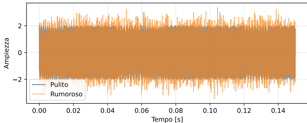
Rumoroso ( \sigma = 1 ) - SNR = 0.0 dB
