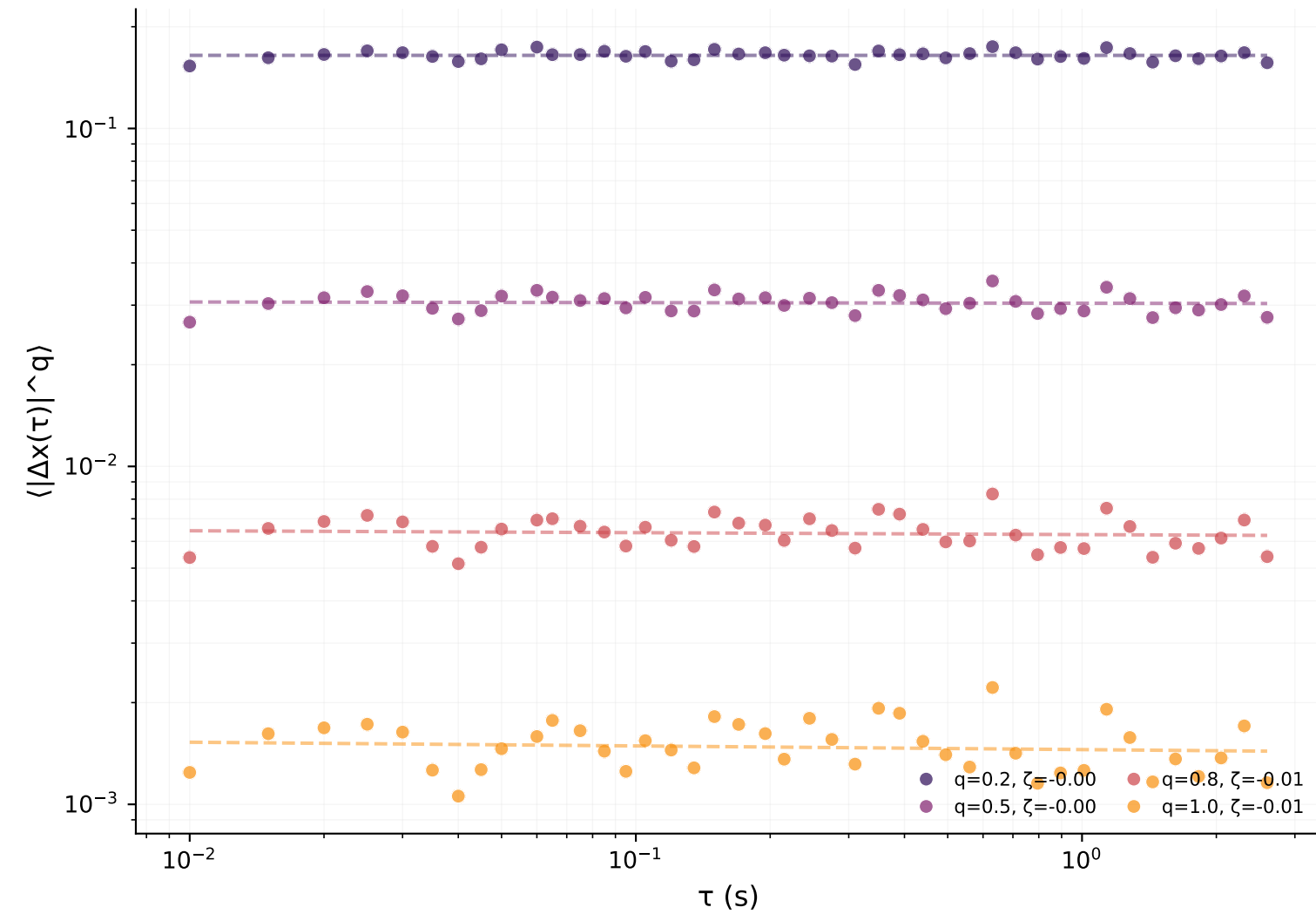
Coda
