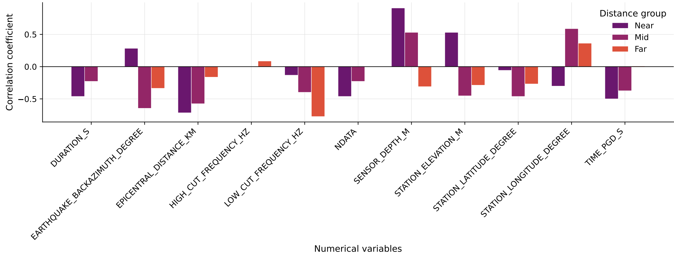
PGD correlation with numerical variables by distance group
