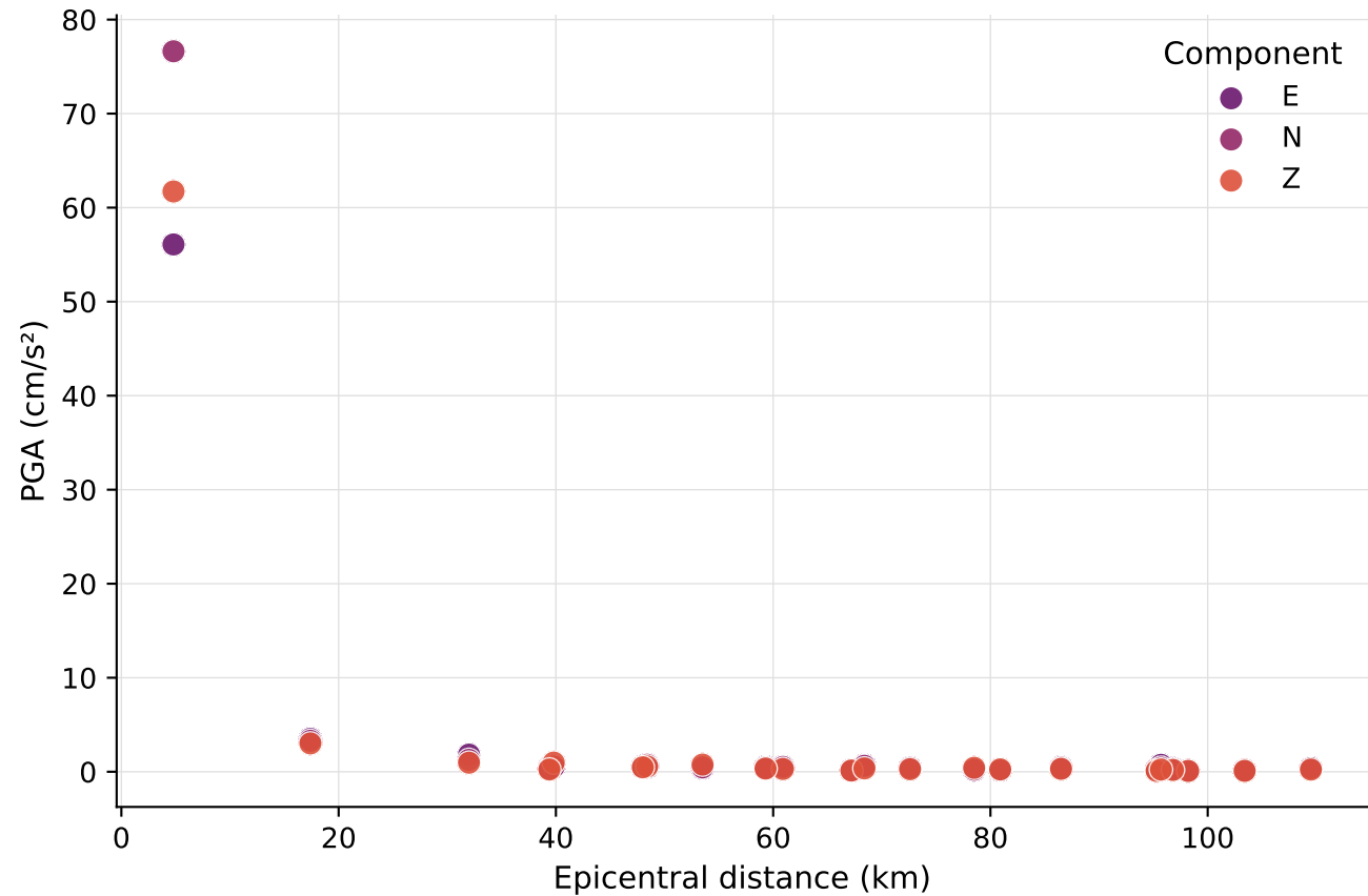
PGA vs epicentral distance by component
