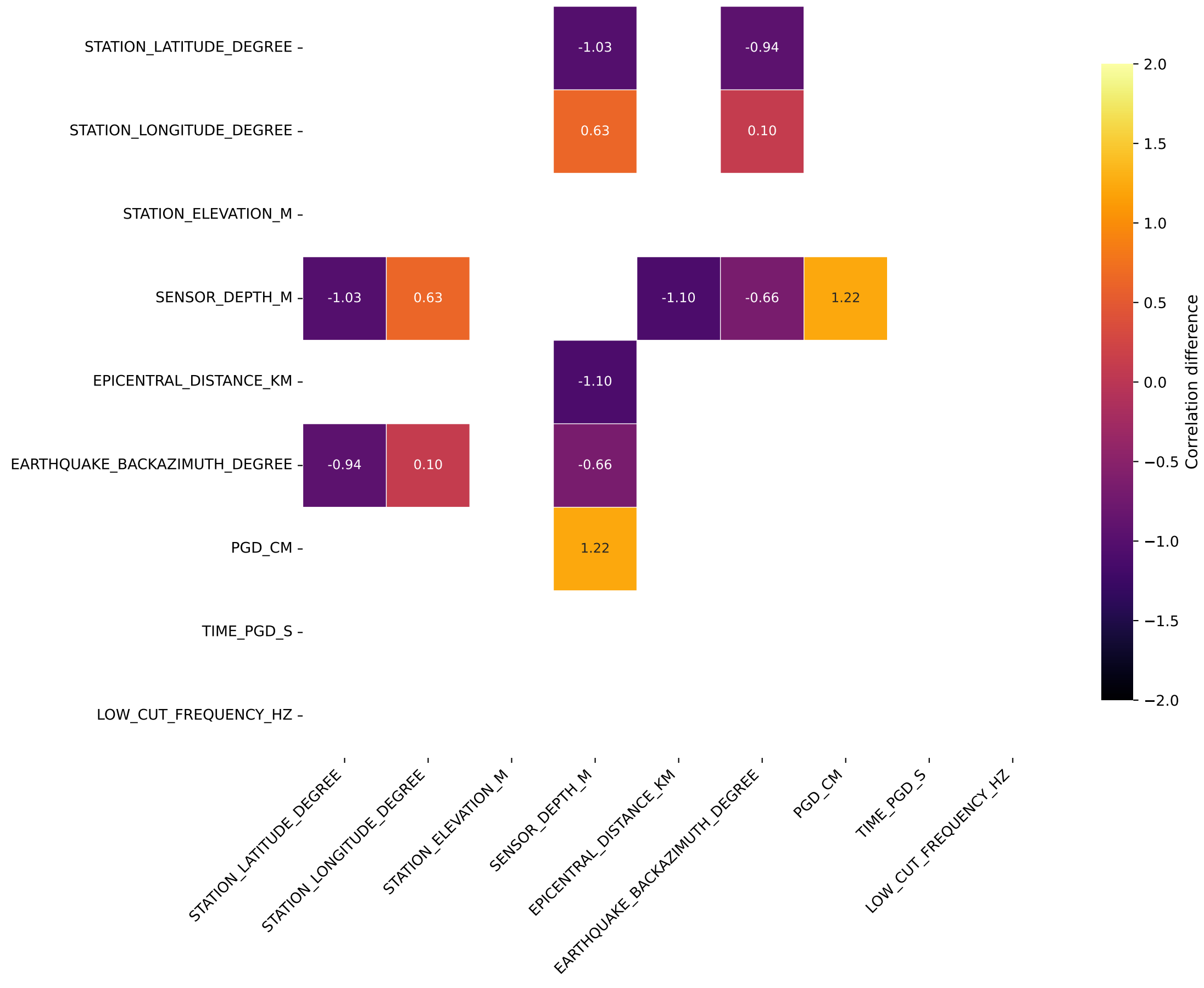
Significant correlation differences ( p < 0.05 ): Near vs Far
