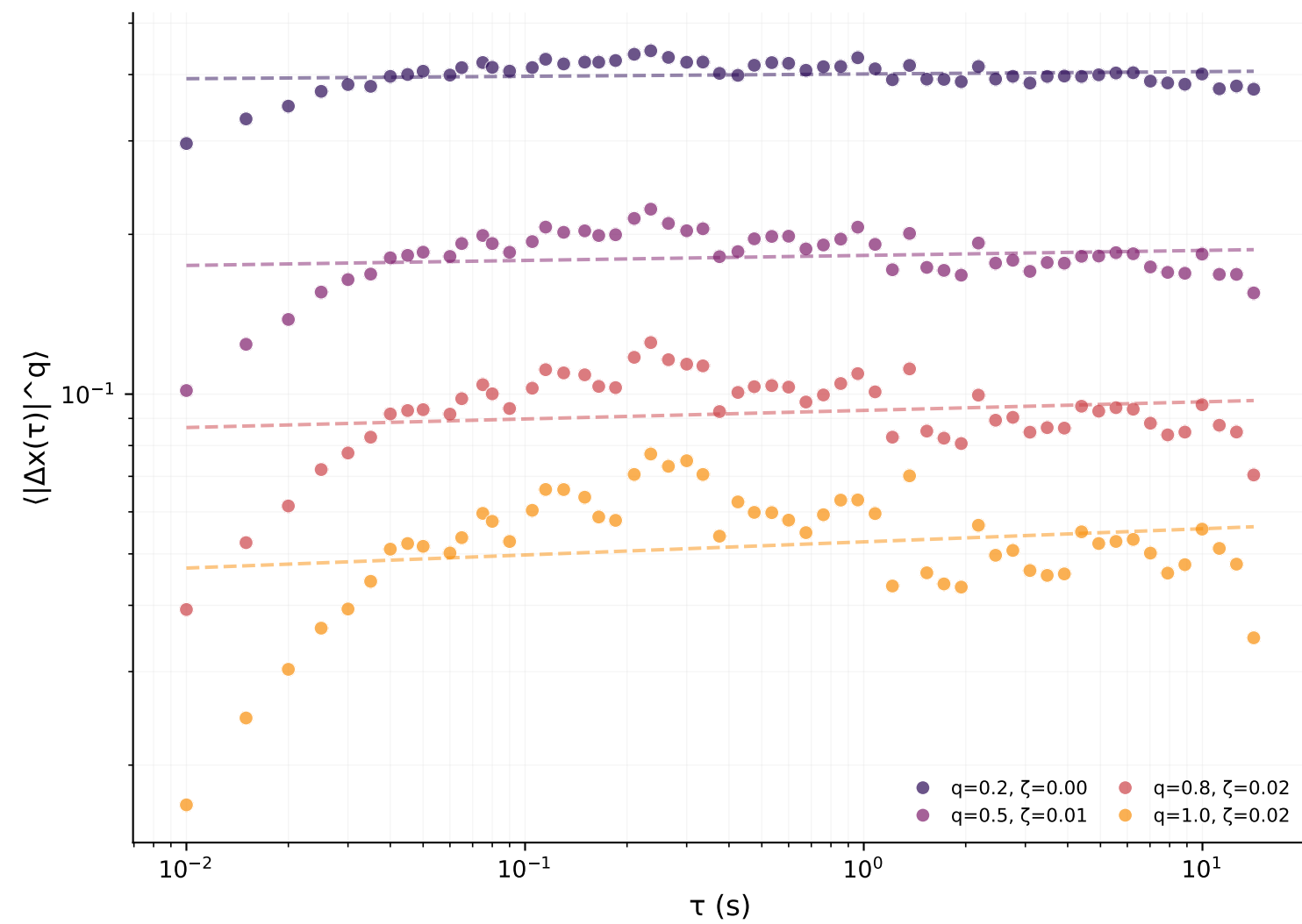
Coda
