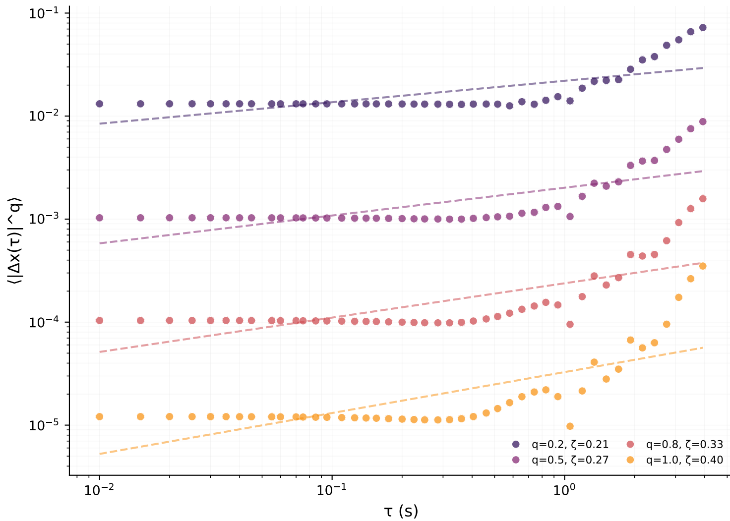
S-wave
