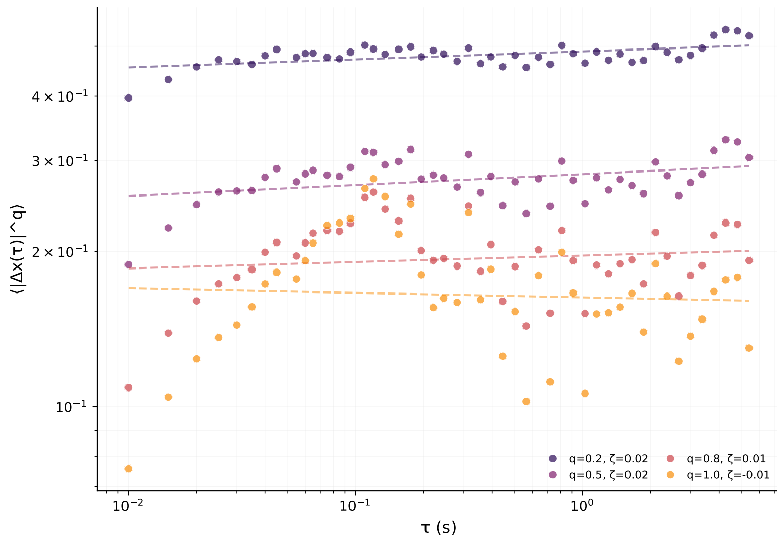
S-wave
