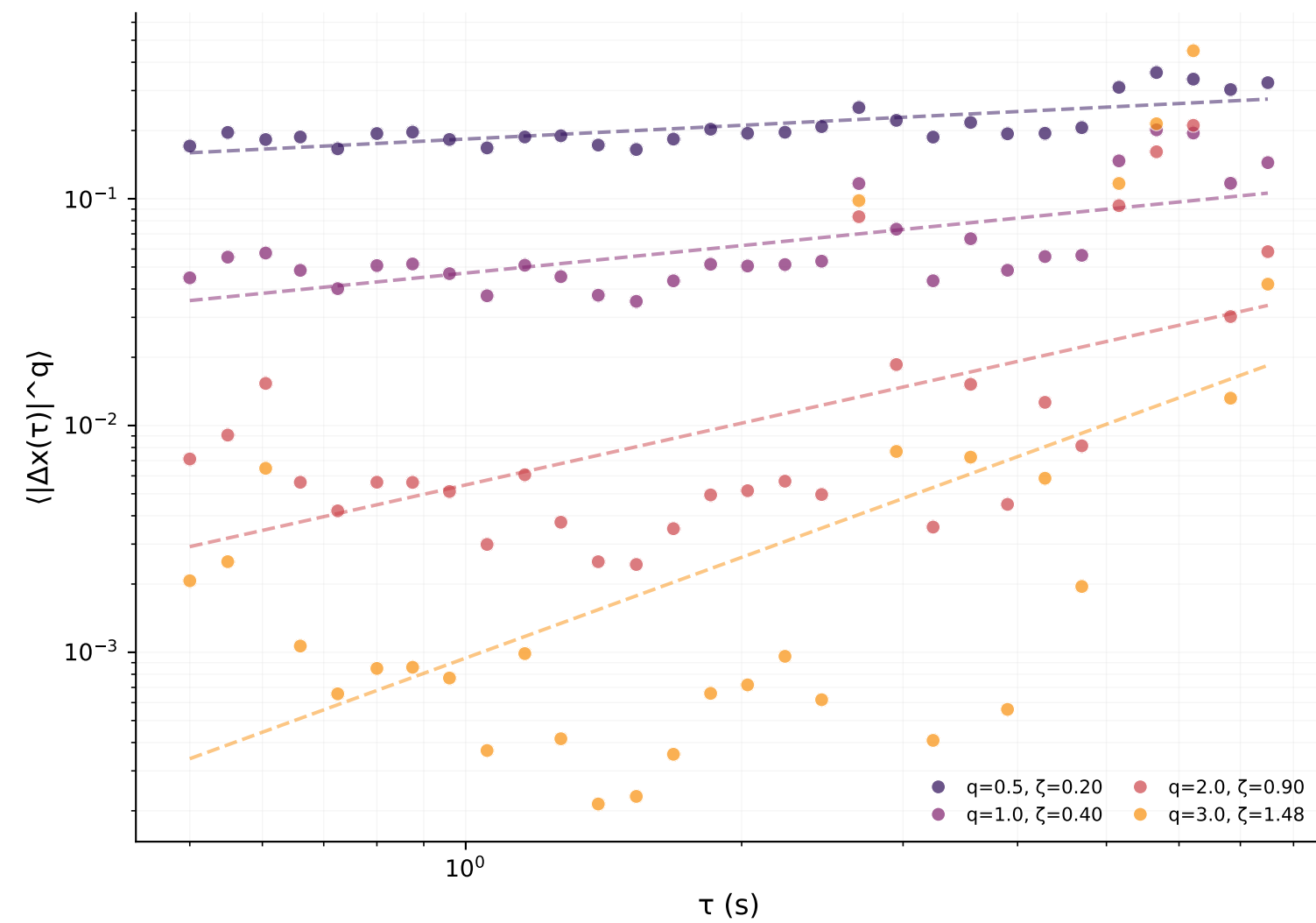
S-wave
