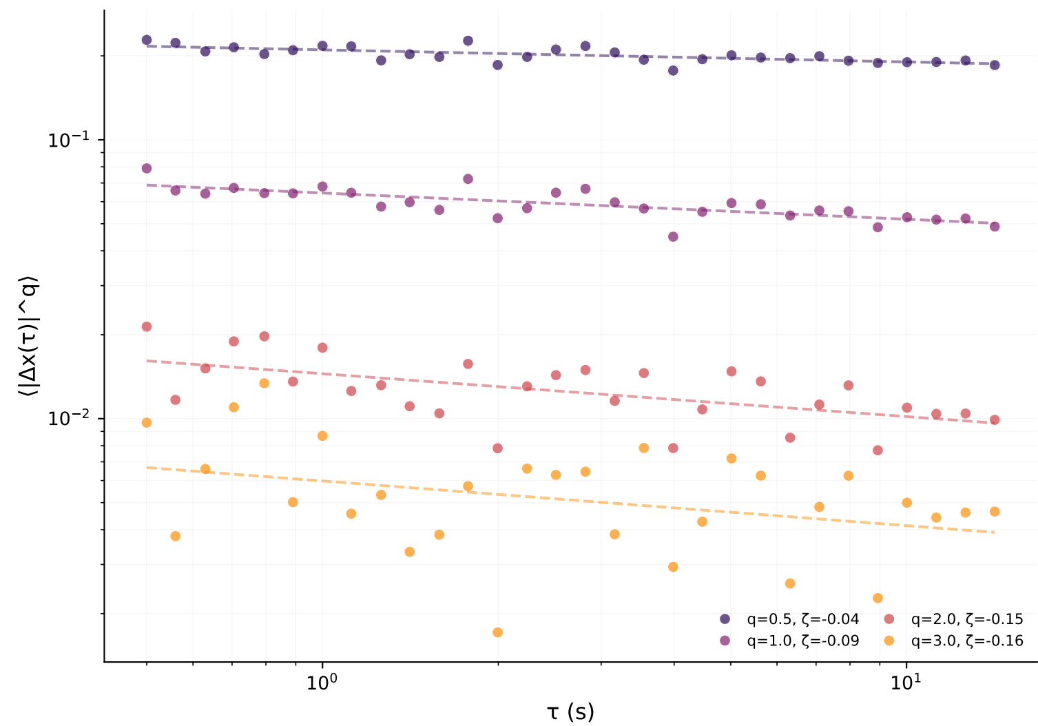
Coda
