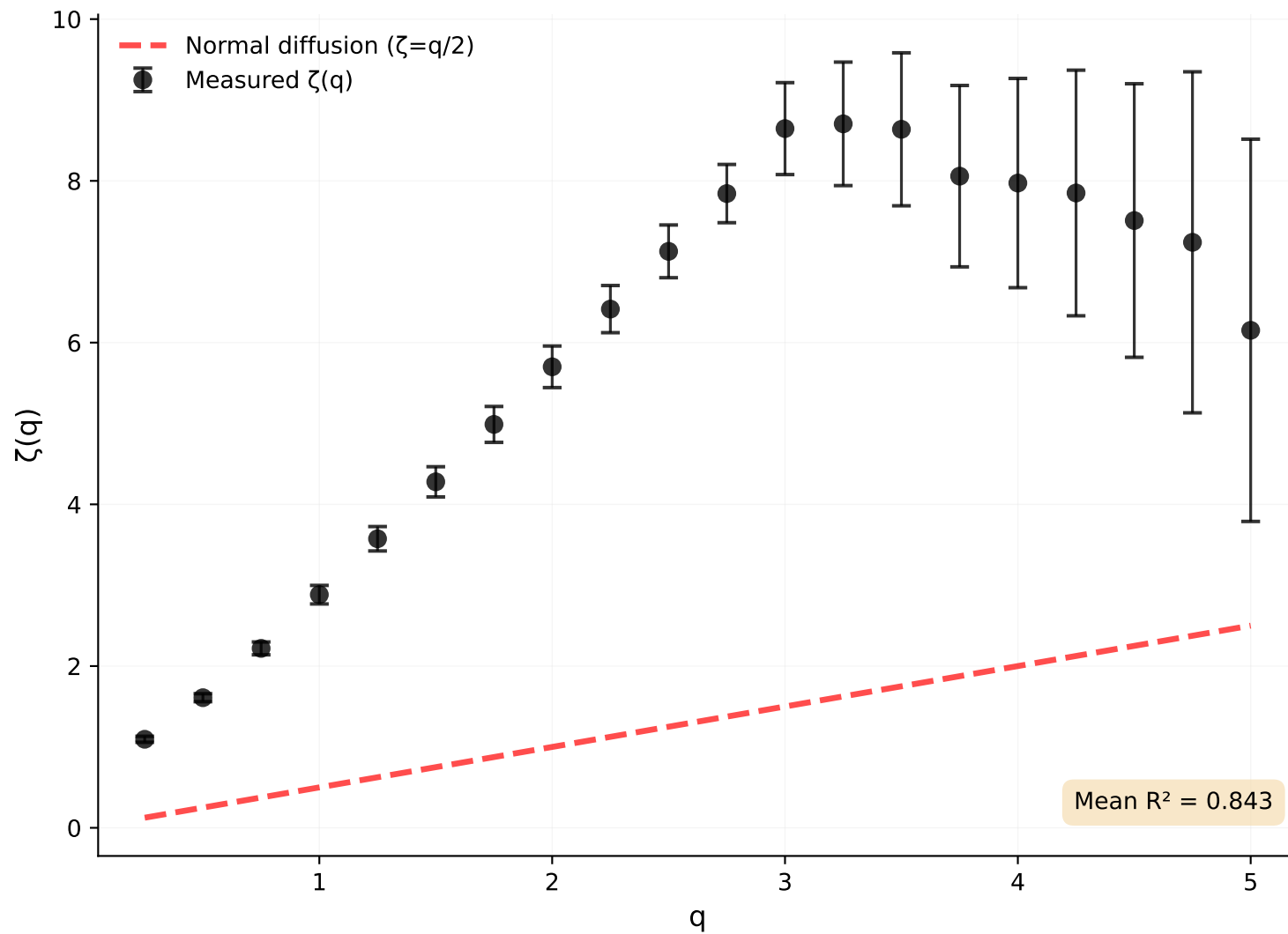
S-wave
