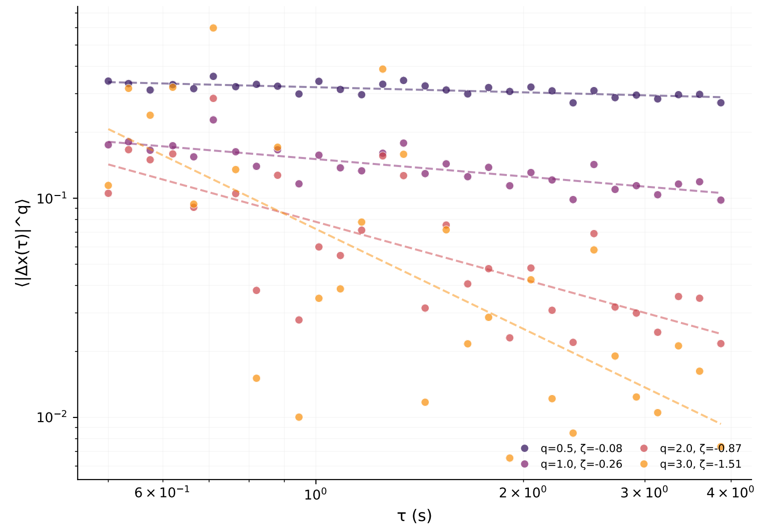
S-wave
