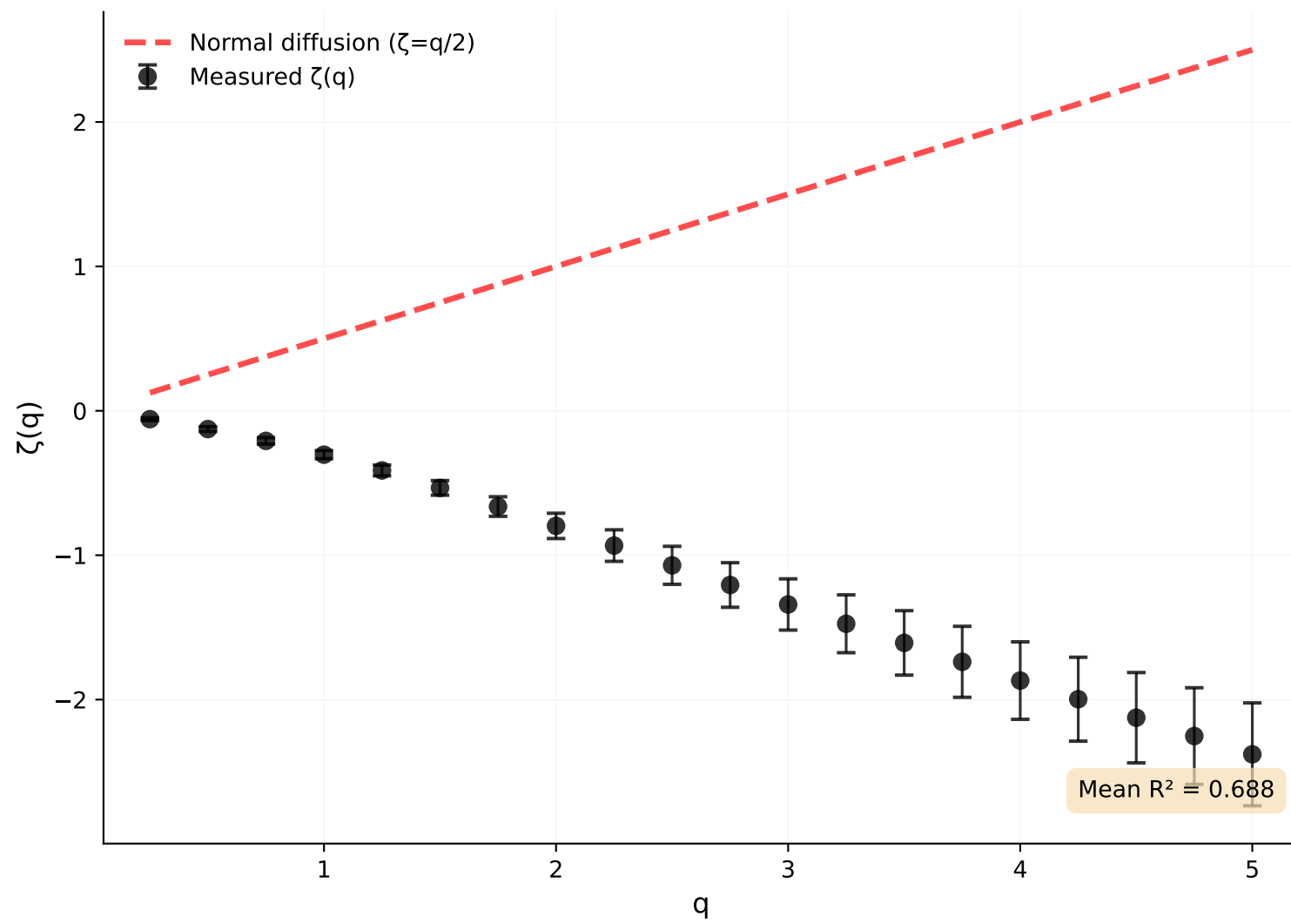
S-wave
