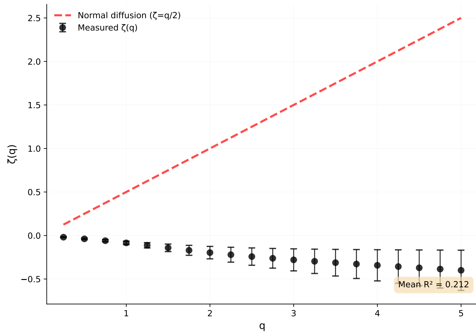
Coda
