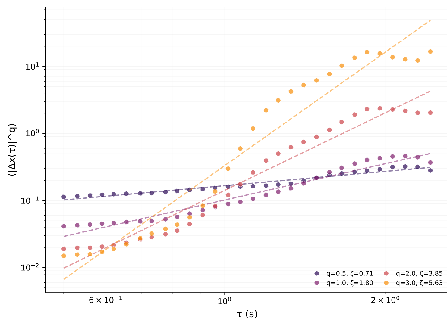
P-wave
