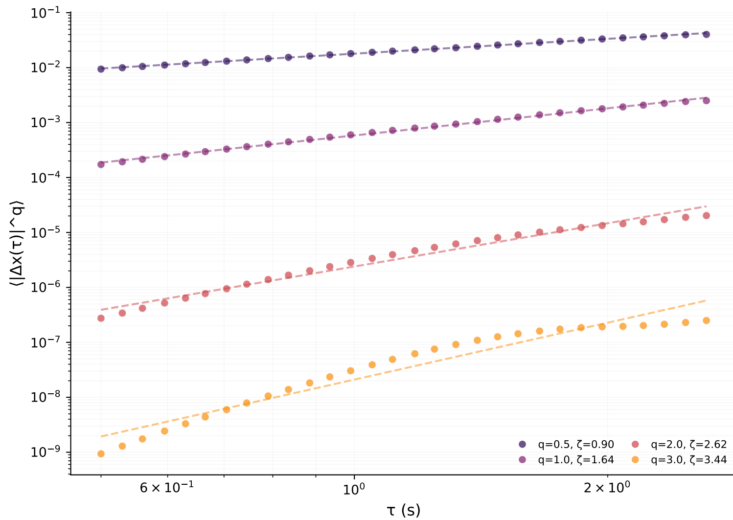
Pre-event (noise)
