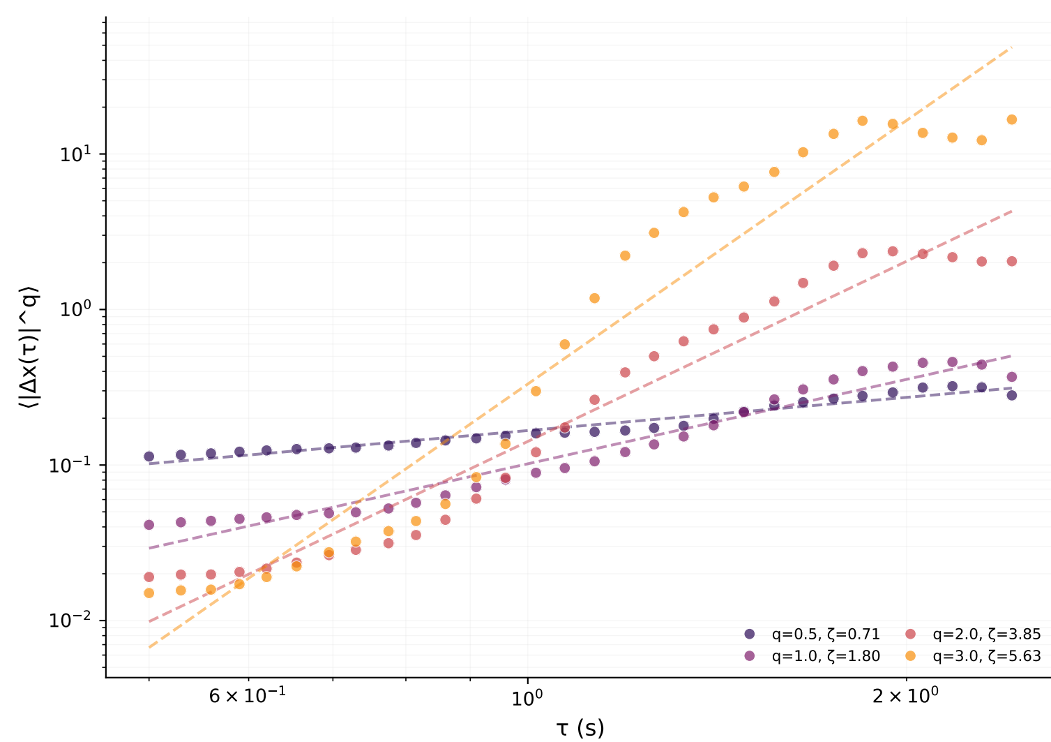
P-wave
