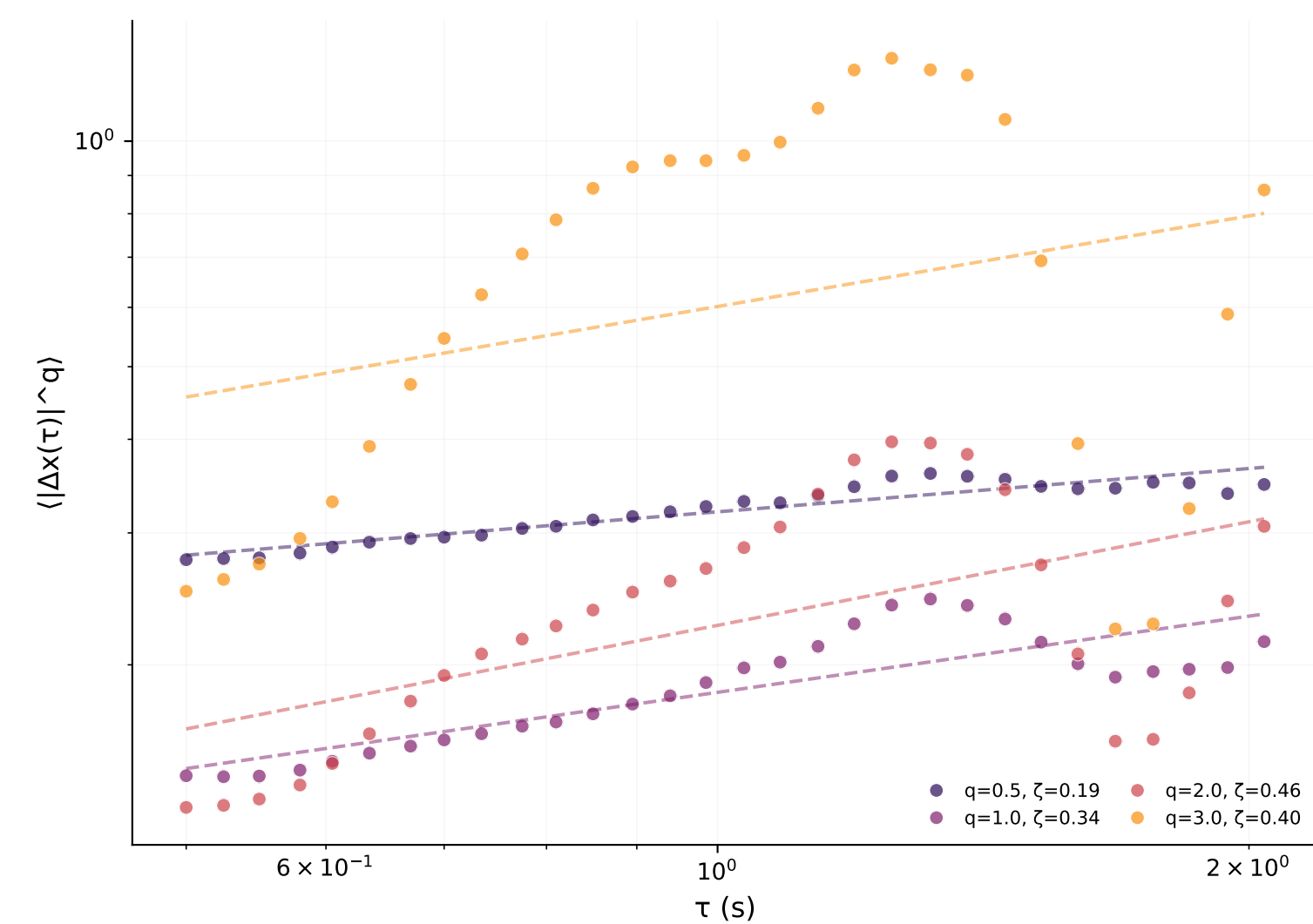
Coda
