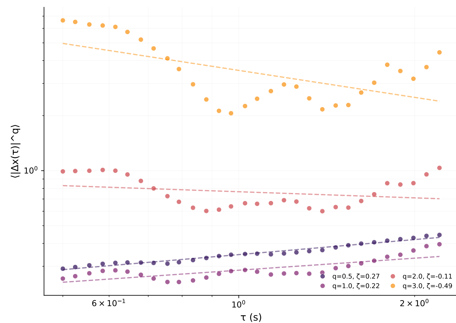
S-wave
